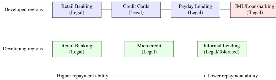
FIGURE A.1: Illegal Money Lending (IML) versus other credit markets.
