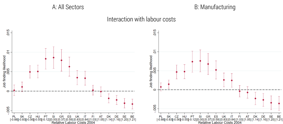
Figure 6: Marginal effects of robot exposure on the likelihood of job finding.
