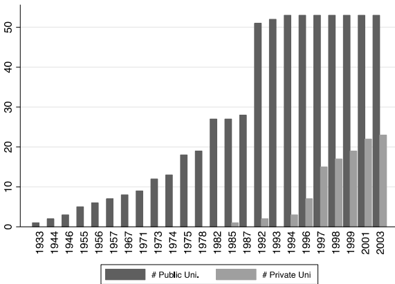
Figure 1: Number of Public-Private Universities
