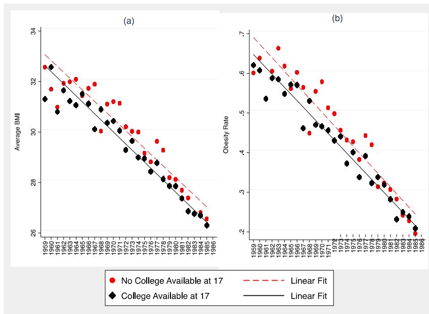
Figure 9: Average BMI and Obesity Rate
