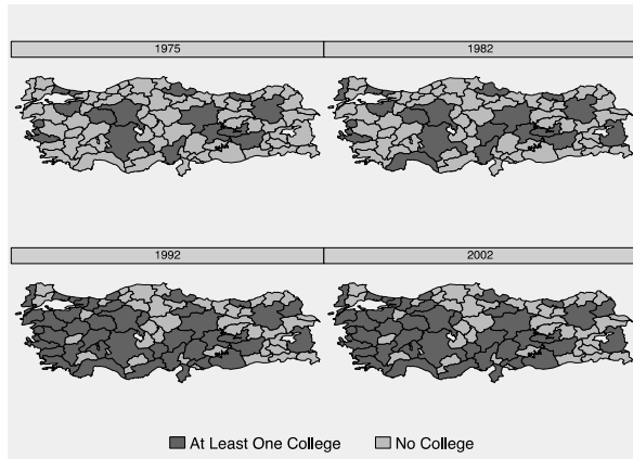
Figure 4: Spatial Distribution of Turkish Provinces With at Least One College Authors' illustration based on Higher Education Statistics of Council of Higher Education (COHE)
