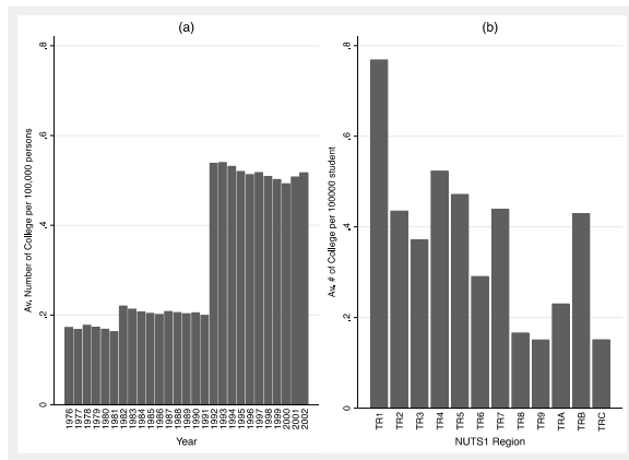
Figure 5: Number of Colleges per 100,000 persons by Year and Region Authors' illustration based on Higher Education Statistics of Council of Higher Education (COHE). (a) shows the average number of colleges per 100,000 persons aged 18-24 by year. (b) shows the average number of colleges per 100,000 persons aged 18-24 by 12 NUTS1 regions between 1975-2002. Number of universities include both public and private colleges.
