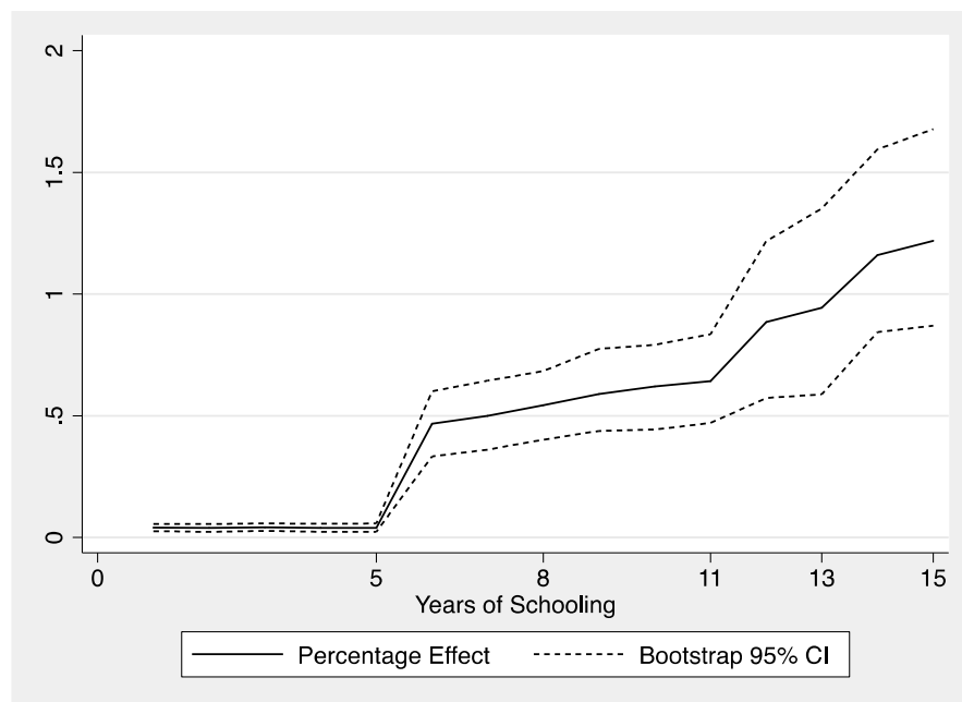
Figure 8: Percentage Effect of College Proximity on the Distribution of Years of Schooling
