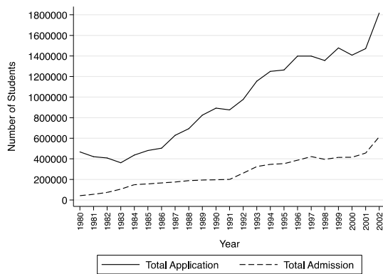
Figure 2: Number of College Applications and Admissions
