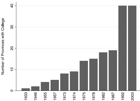
Figure 3: Number of Turkish Provinces with at least One College, by Year
