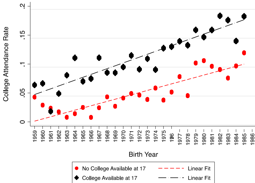
Figure 7: College Attendance Rate
