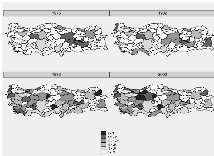
Figure 6: Spatial Distributions Number of Colleges per 100,000 persons Authors' illustration based on Higher Education Statistics of Council of Higher Education (COHE).
