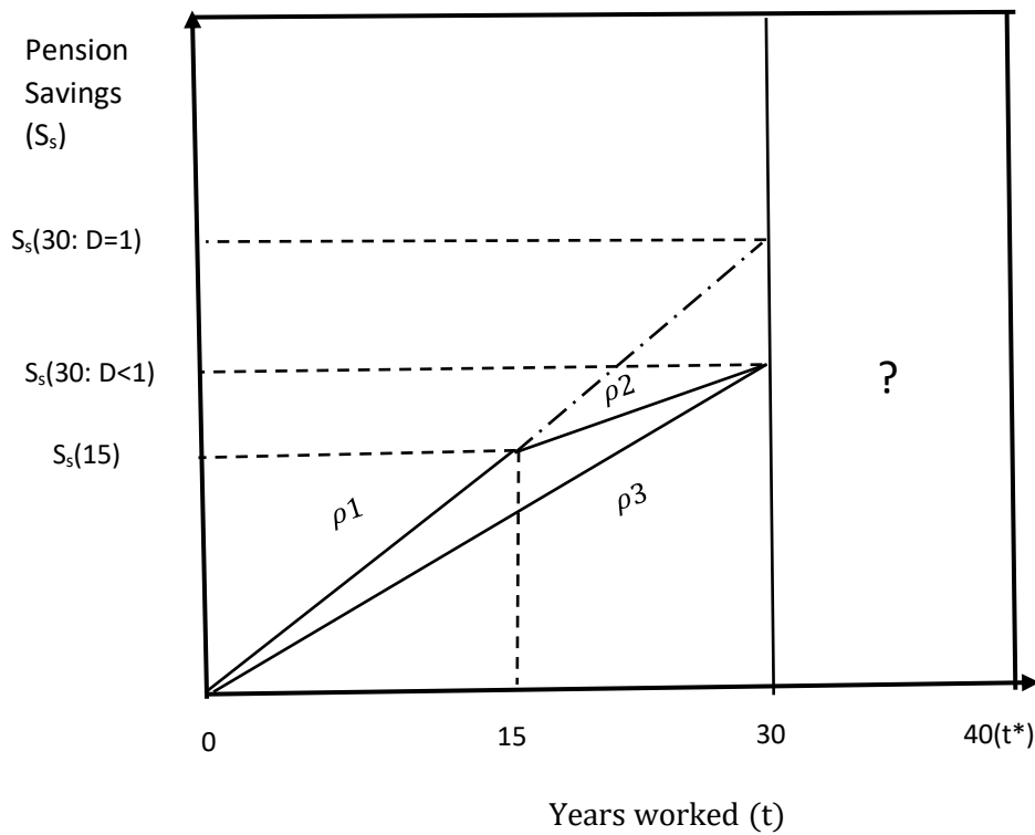
Stylised Pension Savings Model with Individual Decision-making
