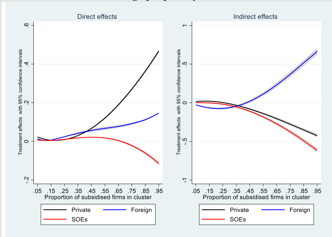
Figure 6: Estimation without firm-specific productivity trends in first-stage propensity score models
