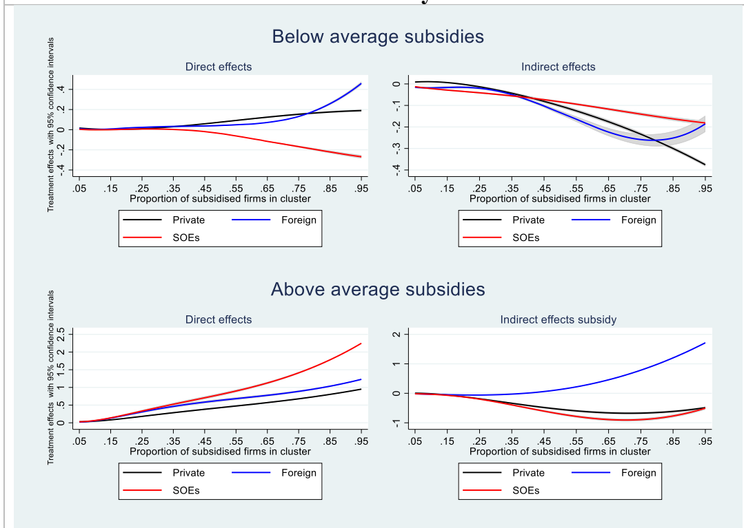
Figure 8: The causal effects of subsidy on productivity by the level of subsidy
