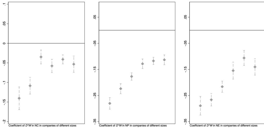
Figure 7 Estimated Coefficients of D \cdot w in Model (2) for Firms of Different Size
