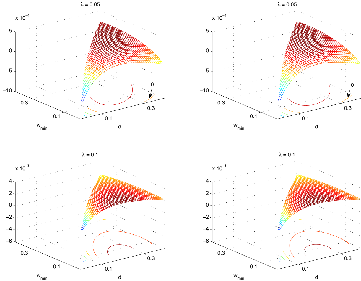
Figure 2: Exact and asymptotic difference in MSFE with T = 1000
