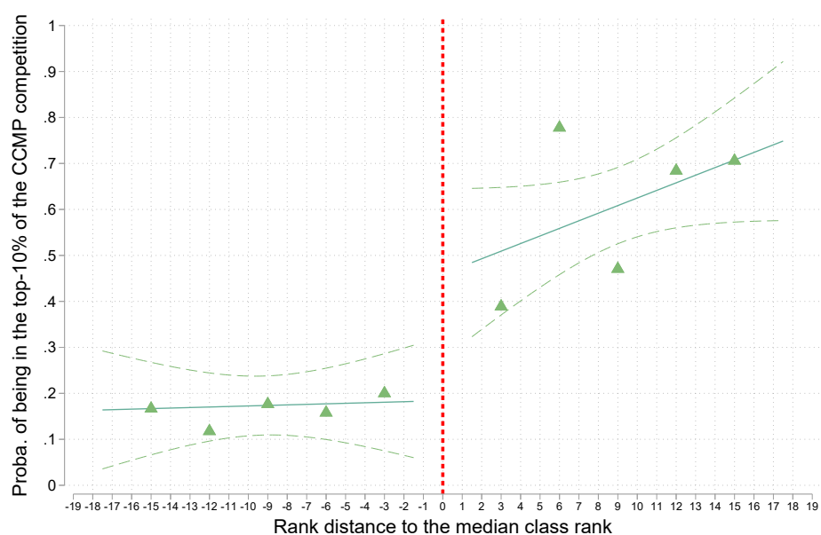
Figure B6: End-of-first-year and probability to score among the top-10% of the CCMP competition
