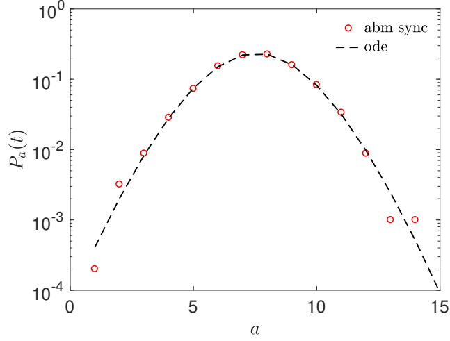
Figure F.1: The log-productivity distribution P_a(t) from a Monte Carlo simulation of the stochastic process indicated with circles. The dashed line indicates the solution of the ODE of Equation (27).
