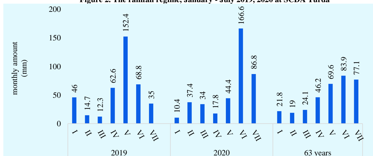
Figure 2. The rainfall regime, January - July 2019, 2020 at SCDA Turda
