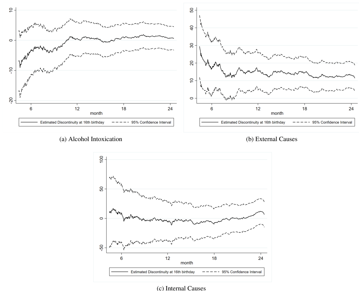
Figure C.9: Robustness to Bandwidth Choice – Hospital Admission Rates at Age 16
