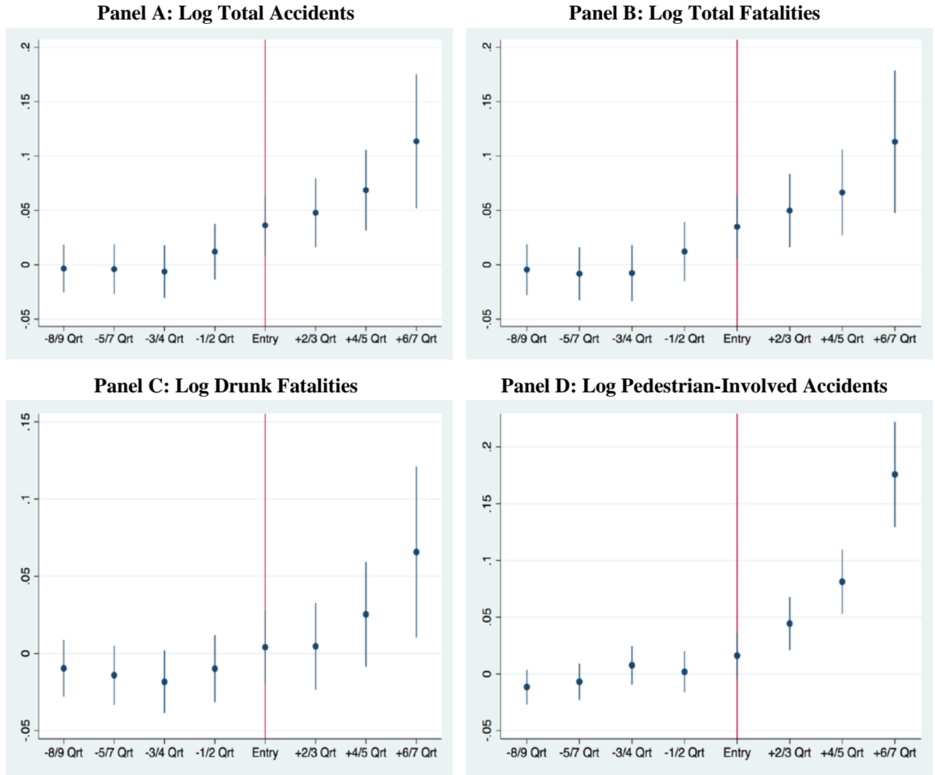
Figure 5 Difference-in-Differences Estimators
