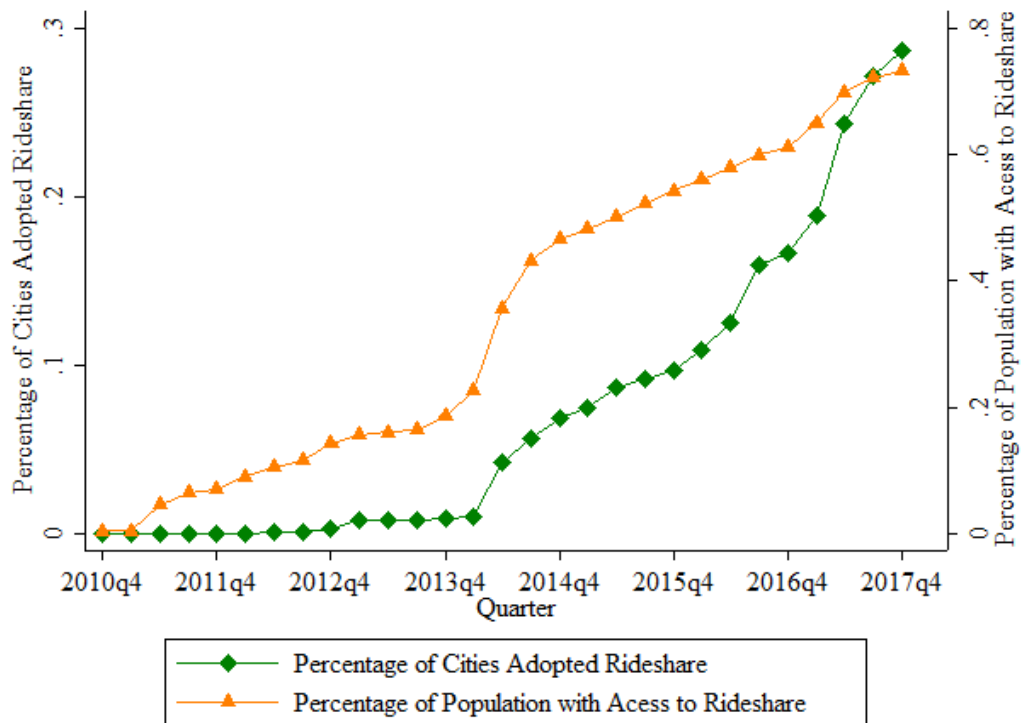
Figure 3 Rideshare Diffusion
