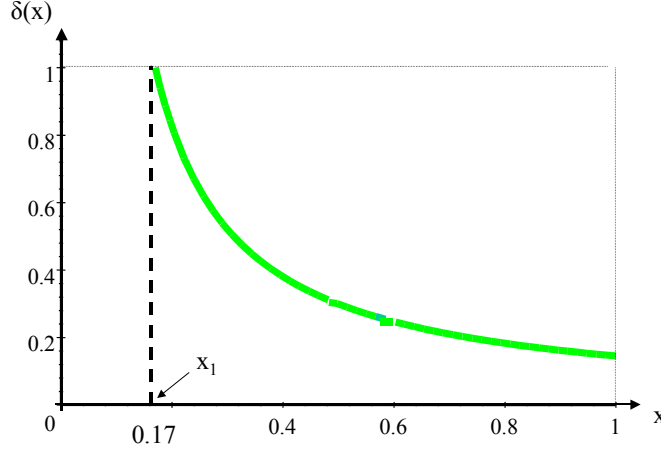
Figure 4: \delta(x) when \lambda = 0.83 and c = 0
