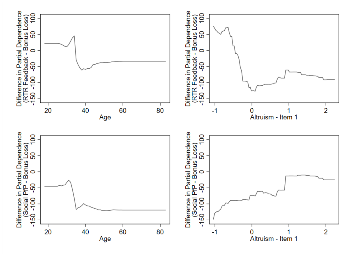
Figure 2: Partial Dependence Comparisons (Example)
