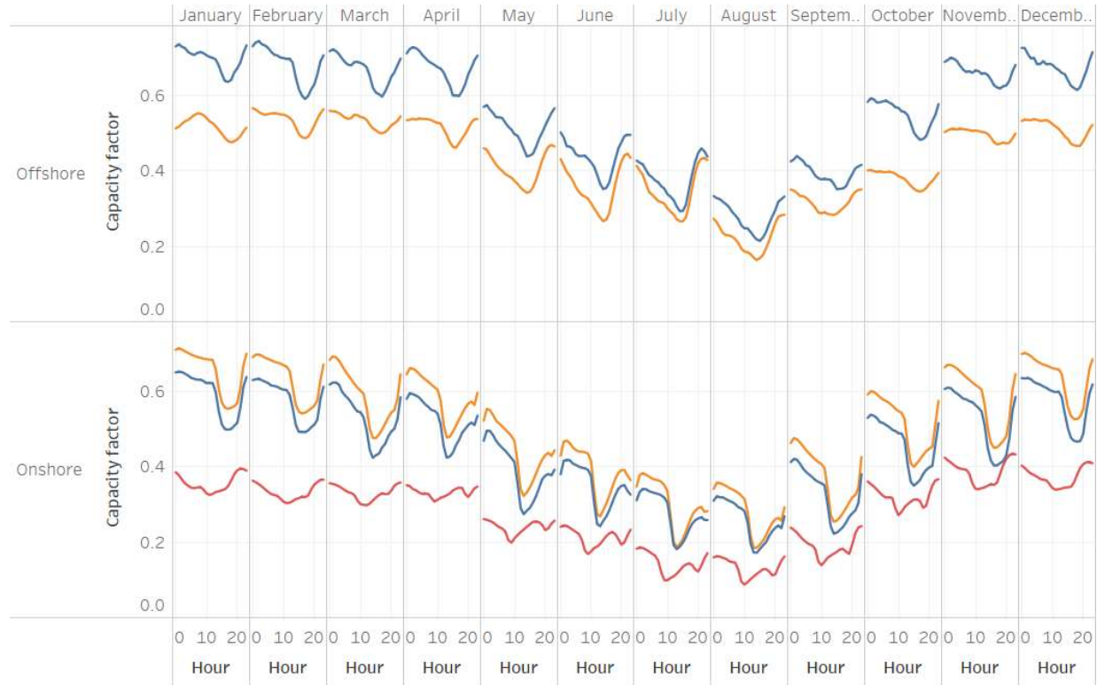
Figure 3.8: Comparison of average capacity factor
