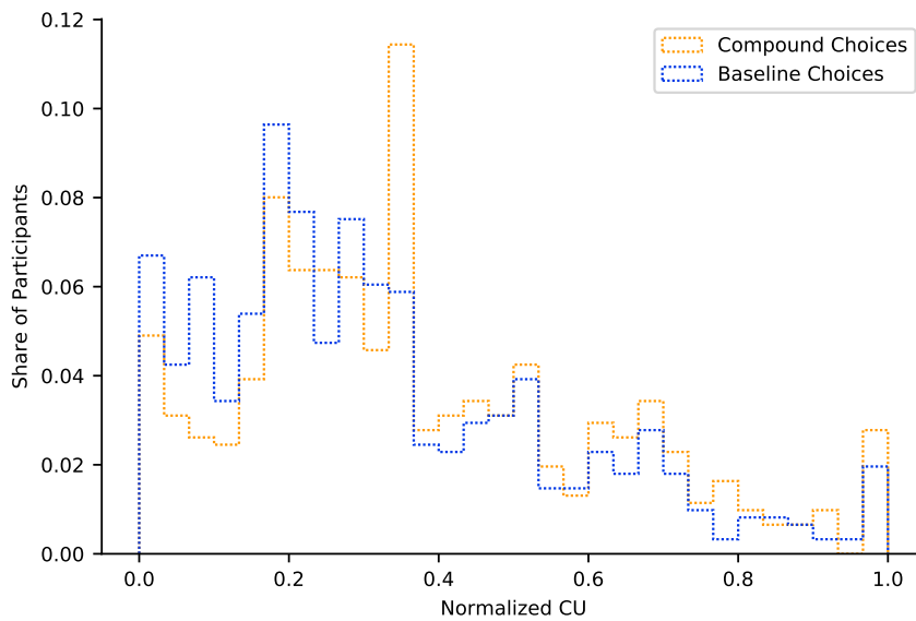
Figure E.1: CU distribution for compound/baseline choices
