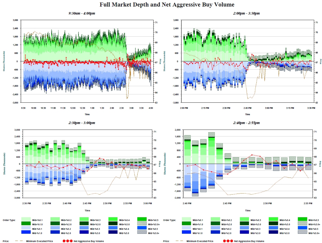
Figure 9: Market Depth and Prices of iShares Russell 2000 Index on May 6, 2010
