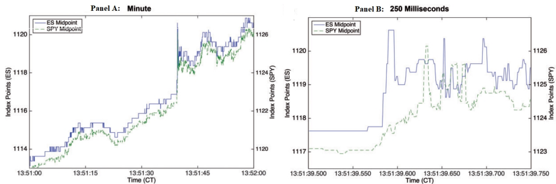
Figure 2: Micro-Structure Price Movements SPY and ES
