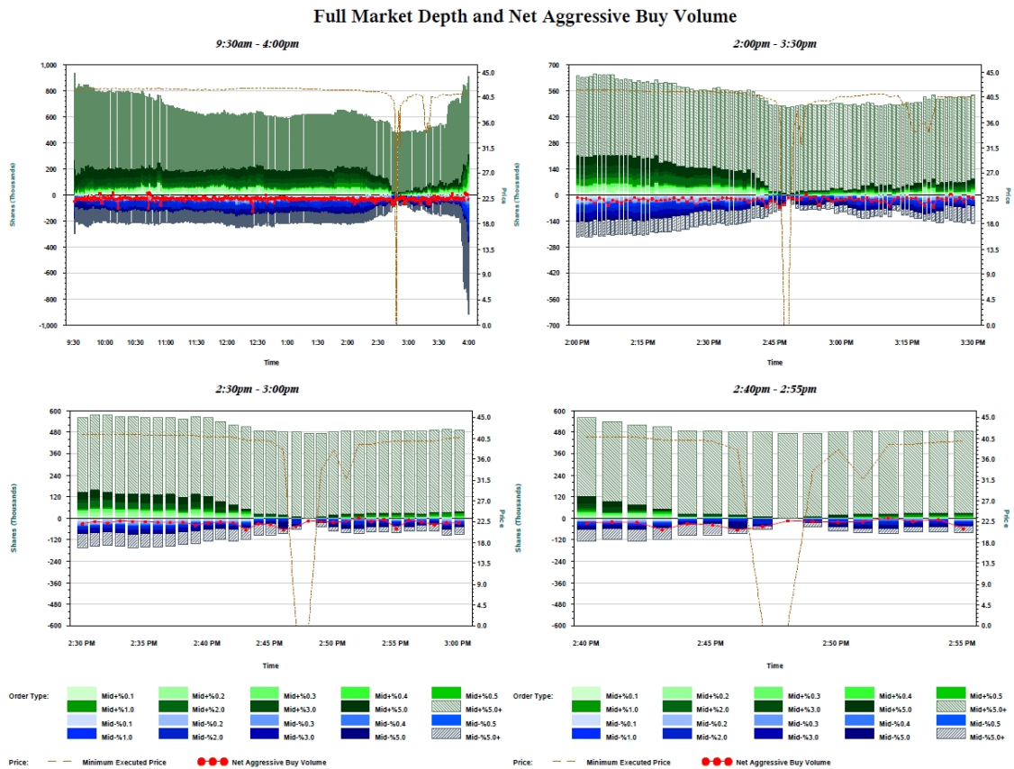
Figure 20: Market Depth and Price Movement of ACN on May 6, 2010
