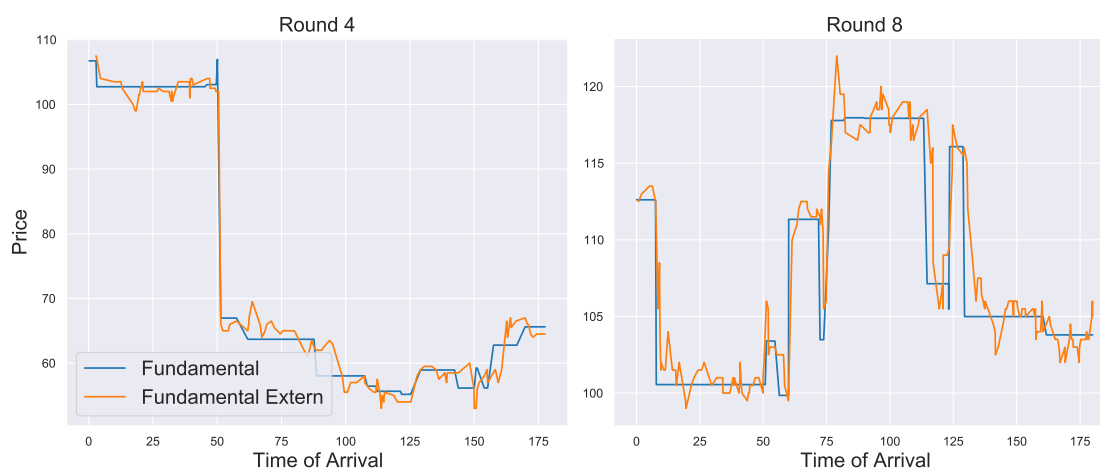
Figure 10: Fundamental values of S3 and S4
