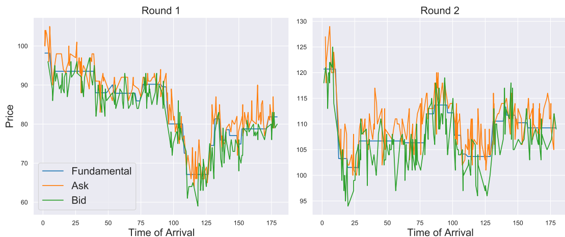
Figure 6: Investors' Orders in Rounds 1 and 2
