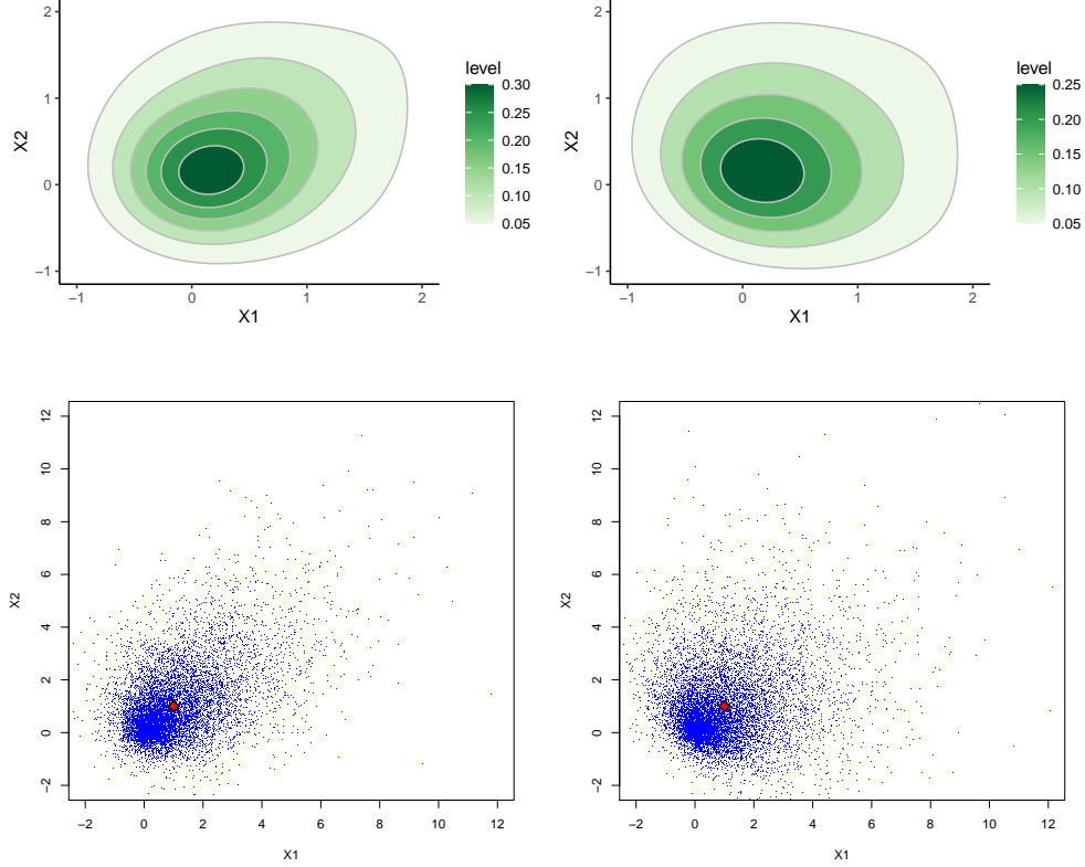
FIGURE 1. Contour plots of bivariate MGAL and MAL distributions of \mathbf{X}_1 and \mathbf{X}_2 in Example 4.1 (top) estimated from 10000 simulated pairs (bottom). Left Panels: the MGAL distribution, constructed via standard univariate gamma scaling with \alpha = 1 , \mathbf{A} = (1 \ 1)^\top , and \mathbf{\Sigma} = \mathbf{I}_2 . Right Panels: the MAL distribution, constructed via matrix variate gamma scaling with \alpha = 1 , \mathbf{A} = (1 \ 1)^\top , and \sigma^2 = 1 . The diamond in the bottom figures marks the mean vector. Its location relative to the mode illustrates skewness of the distributions.
