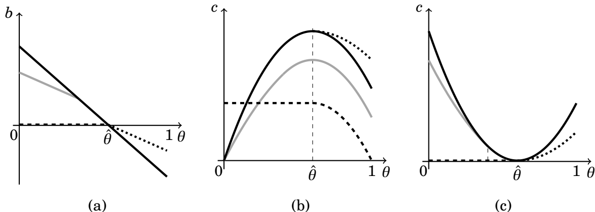
Figure 3: Illustration of Proposition 4.1. Subfigure (a) plots four biases, all inward with respect to \frac{3}{5} , where the gray, dashed and dotted line are biases resulting from local reductions of the black line. In (b) we depict the corresponding coarseness of communication. In (c) we depict the coarseness of communication corresponding to switching the roles of the agents, that is, multiplying by -1 all the biases.
