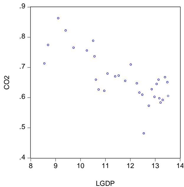
Figure 1: Scattered plot for CO2 per Capita and \ln GDP per Capita in Nigeria
