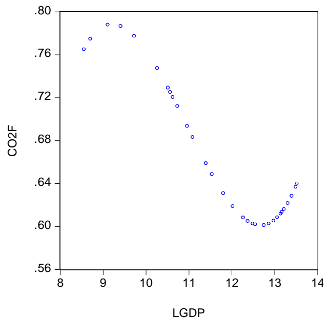
Figure 2: Scattered plot for fitted CO2 per capita and \ln GDP per capita in Nigeria
