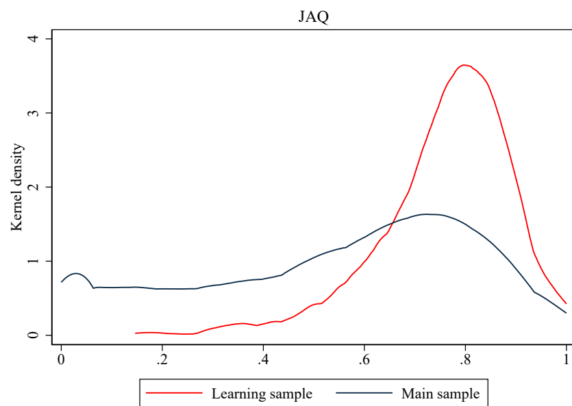
Figure 3: The distribution of JAQ
