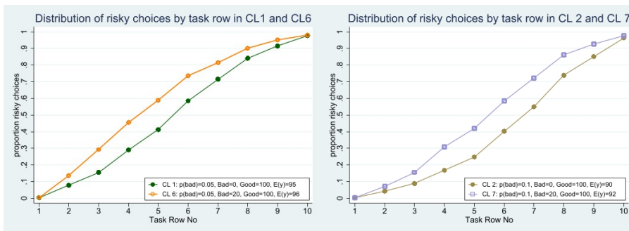
Fig. 4 The distribution of switch points in CL1 vs. CL6 and CL2 vs. CL7.
