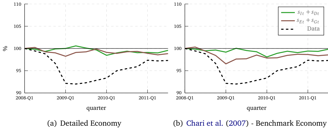
Figure 8: Robustness to the Chari et al. (2007) benchmark economy
