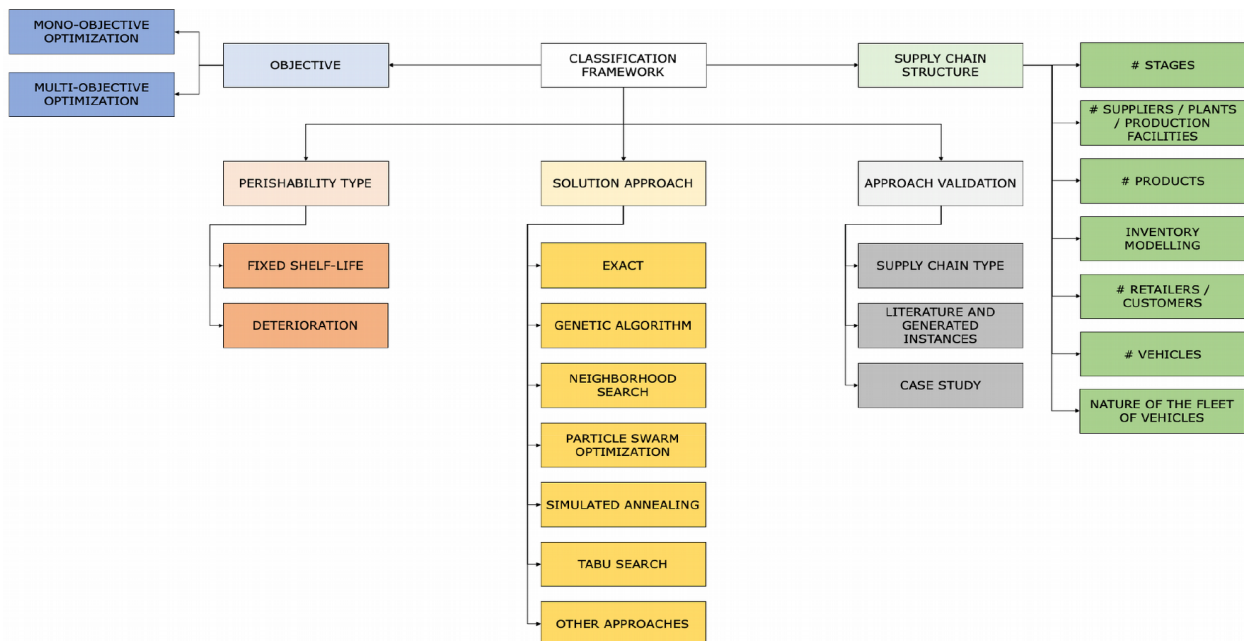
Figure 4. Classification framework
