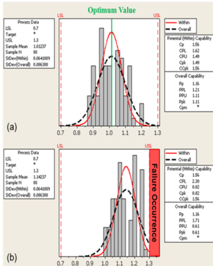
Figure 17. Process capability of trace top/bottom ratio (a) robust design with CPM and (b) uncontrolled system design with occurrence of failure
