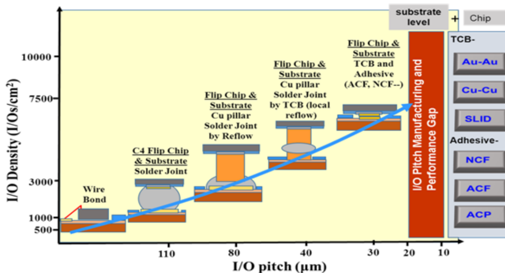
Figure 3. Trend of high-density interconnect (HDI) to support advanced package development
