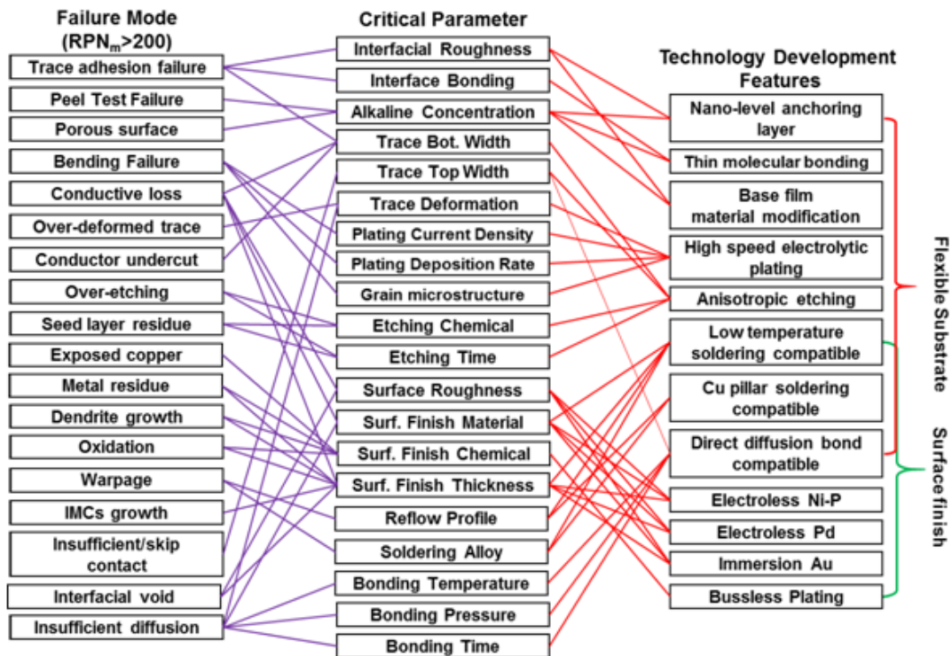
Figure 16. Correlation between high priority failure mode, critical parameter, and technology development features
