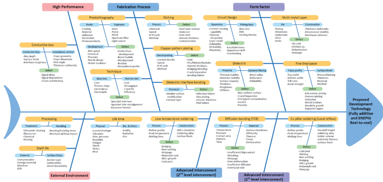
Figure 12. Factors and failure mode of the proposed technology development
