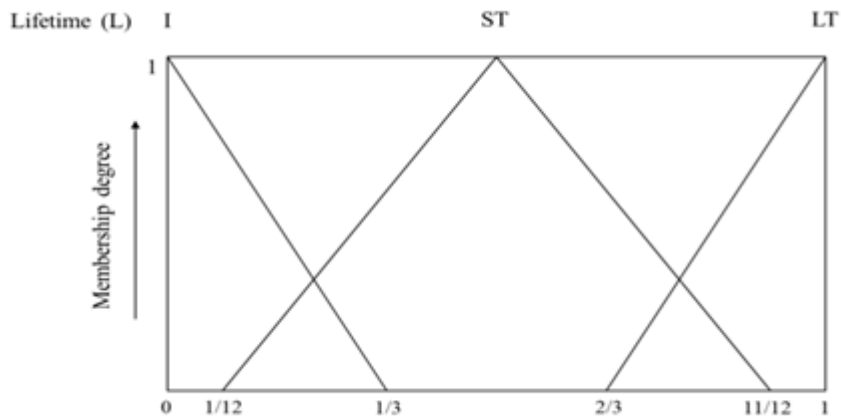
Figure 14. Fuzzy linguistic membership function for lifetime
