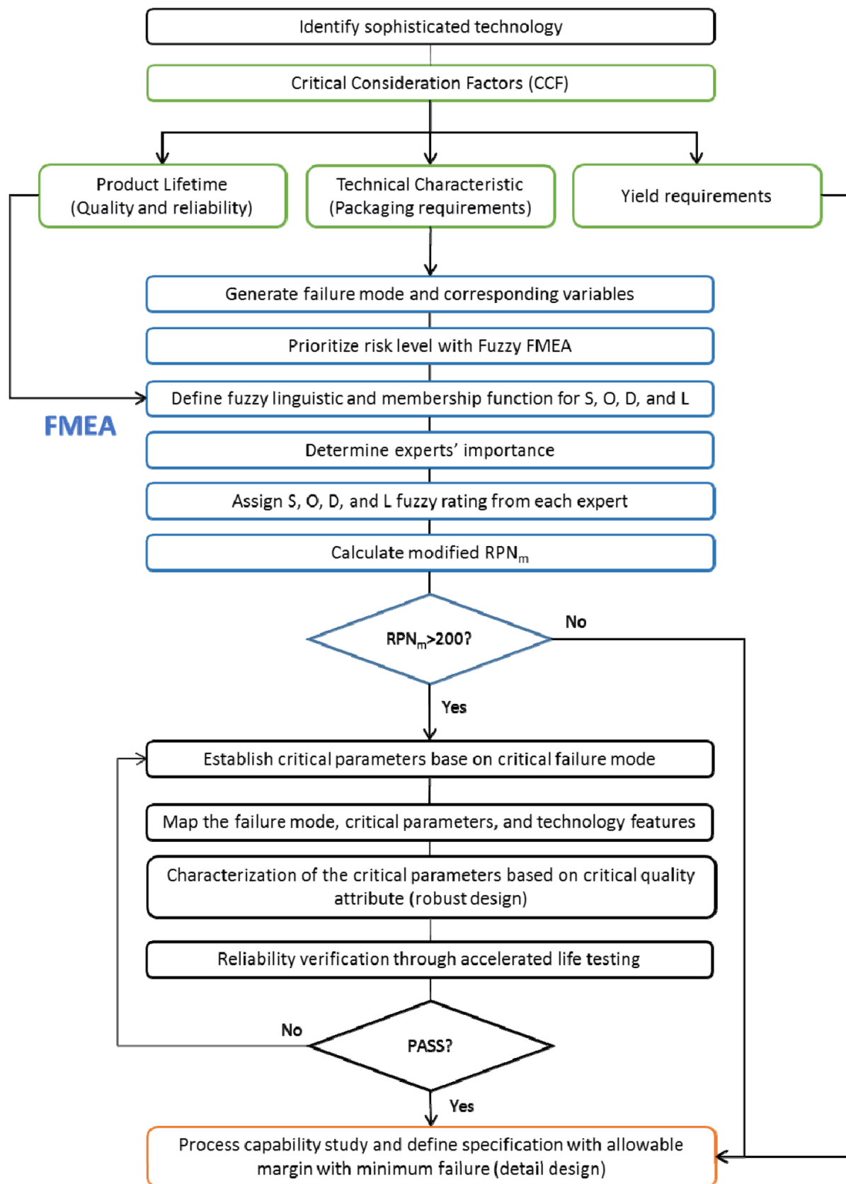
Figure 10. Flowchart on the implementation of the proposed development tools
