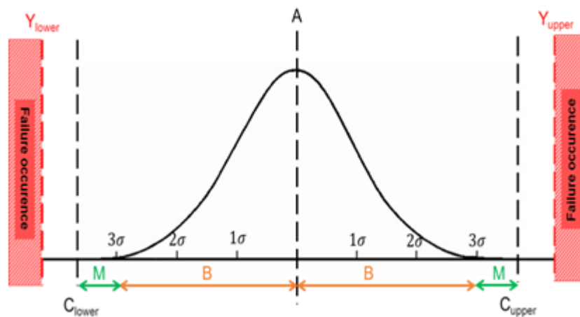
Figure 18. Detailed specification based on process capability
