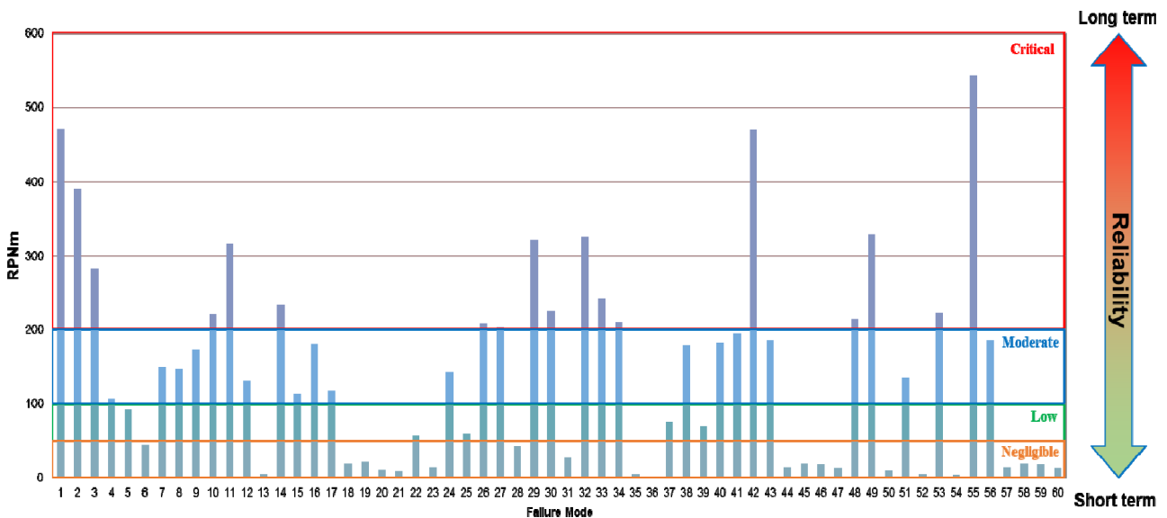
Figure 15. Failure mode RPN in the development of advanced flexible substrate
