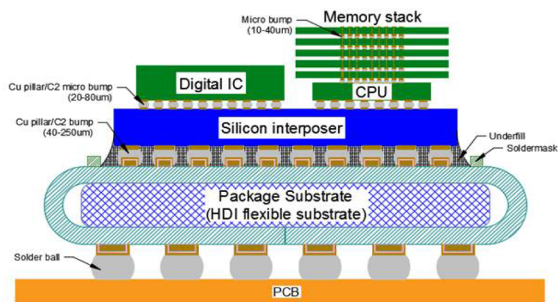
Figure 2. Heterogeneous integration in an advanced electronic package (Pun, Islam, Rotanson, Cheung & Chan, 2018a)
