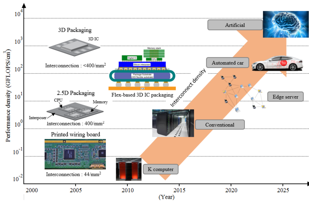
Figure 4. Device packaging technology for servers (Aoki, 2017)
