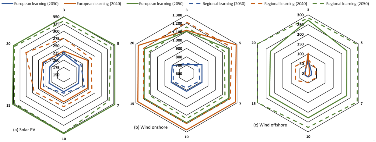
Figure D.1: Installed solar PV (a), wind onshore (b), and wind offshore (c) capacities (in GW) for European and regional learning for different line segments numbers (3, 5, 7, 10, 15, and 20) and periods (2030, 2040, 2050)
