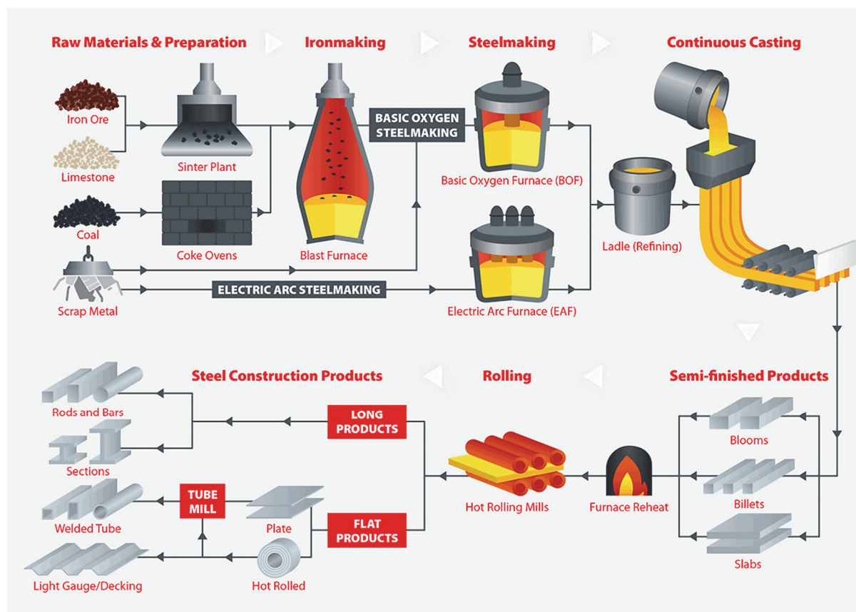
Figure 1: Process of Steel Production
