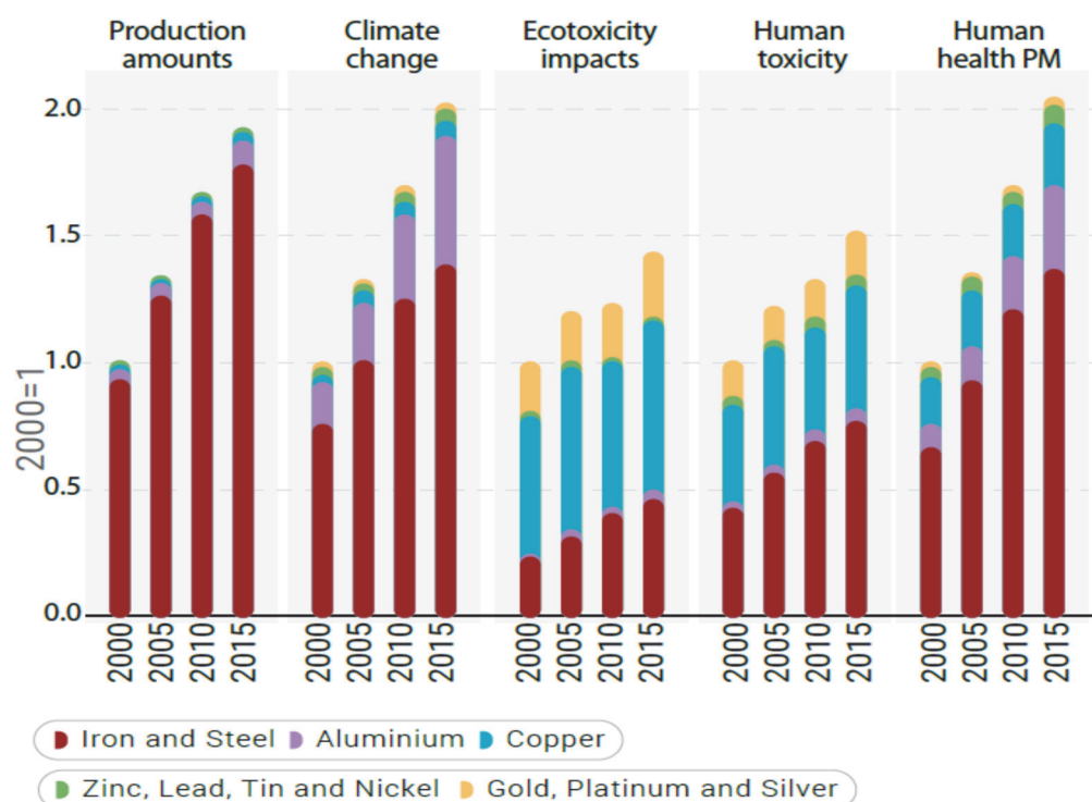
Figure 8: Environmental impacts of metal mining 16
