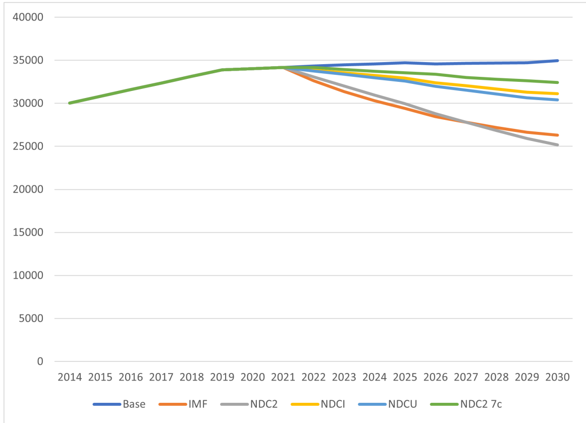
Figure 1: Emission paths until 2030 under different scenarios: NDC targets are insufficient to stay on 2 degrees global warming trajectory
