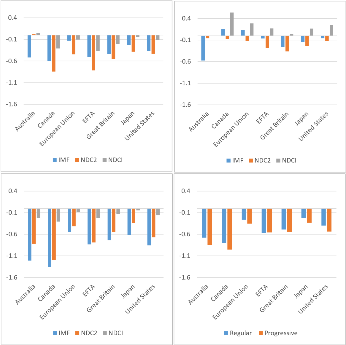
Figure 15: The change in the real income of developed countries when introducing carbon pricing together with complementary measures (clockwise, BCA, Nordhaus, emission trading and Rajan’s incentive scheme)
