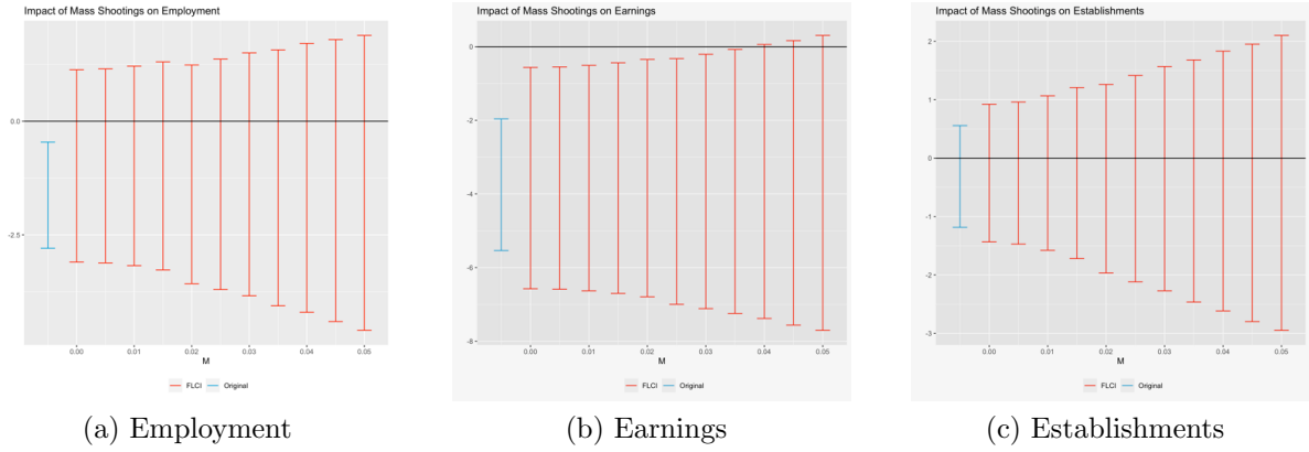
Figure 3: Robustness of Parallel trends assumption
