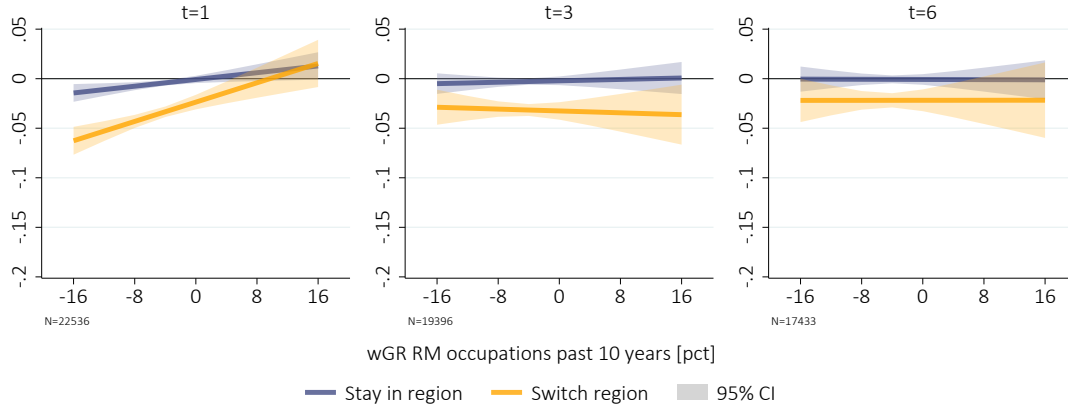
(b) AKM Establishment FE of Region Stayers vs. Switchers
