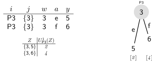
FIGURE 2.4. The 5-form game (Q^1, U^1) . Q^1 is the set consisting of the upper table's rows, and U_{P3}^1: \mathcal{Z}^1 \rightarrow \mathbb{R} is defined by the lower table. The tree diagram provides the same data.
