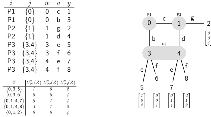
FIGURE 2.5. The 5-form game (Q^2, U^2) . Q^2 is the set consisting of the upper table's rows, and U^2 = \langle U_i^2: \mathcal{Z}^2 \rightarrow \mathbb{R} \rangle_{i \in I^2} is defined by the lower table. The tree diagram provides the same data.
