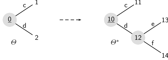
FIGURE 2.4. The morphism [\Theta, \Theta^*, \tau] defined by \tau(x)=x+10 . [\Theta, \Theta^*, \tau] is not end-preserving.
