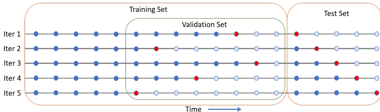
Figure 3: Schematic of expanding window approach for (1-fold) cross-validation and out-of-sample prediction. The available data are divided into training, validation, and test sets. For the given iterations of the expanding window (Iter), ● represents in-sample training points and ● represents out-of-sample test points. For each iteration in the cross-validation, we use randomly sampled ● points from the validation superset as the validation subset. Note: the size of each validation subset is kept similar to the test set.
