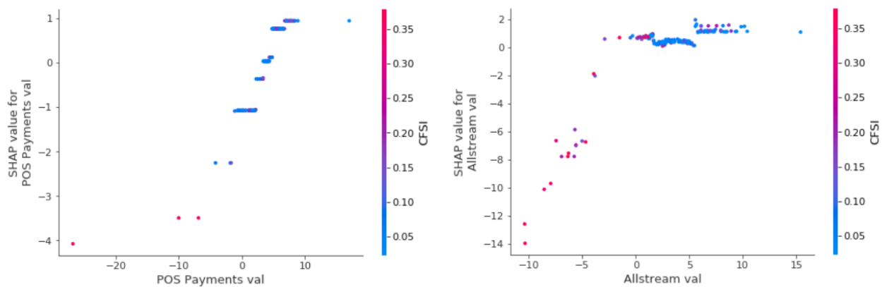
Figure 9: Dependence plots show the Shapley value for each instance in the sample and corresponding predictor value. On the left we show a dependence plot of RTS for the POS payments value, and on the right we show the dependence plot of WTS for the ACSS Allstream value.
