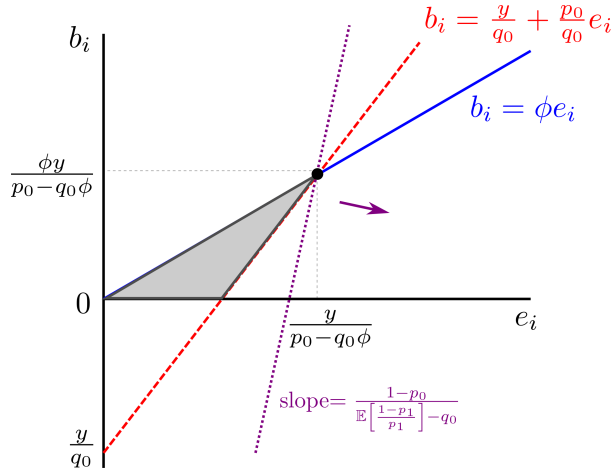
Figure 2: Date 0 problem for FI's
