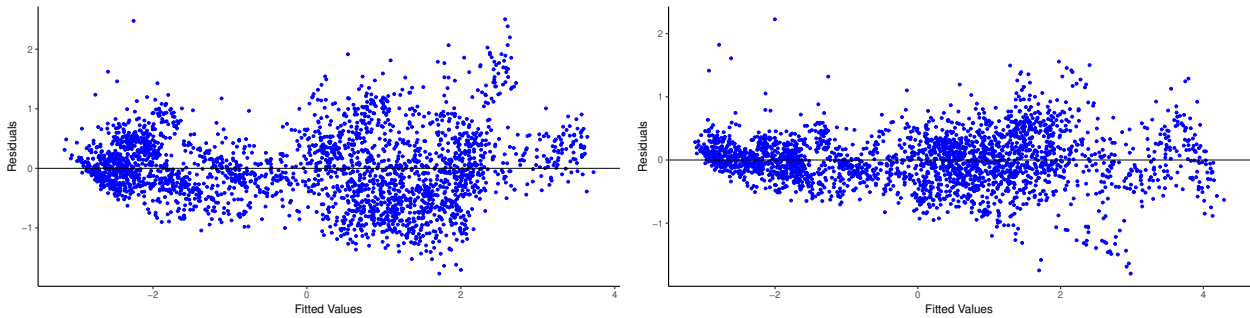
Figure 5: Heteroskedastic Errors
