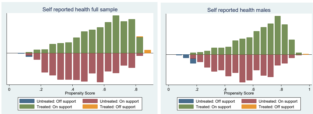
Figure A.1 Propensity score distributions and common support regions
