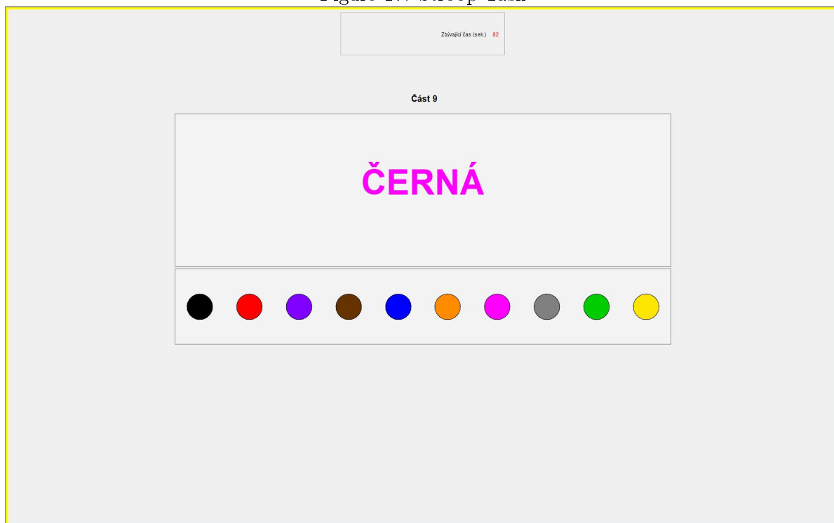
Figure 17: Stroop Task
