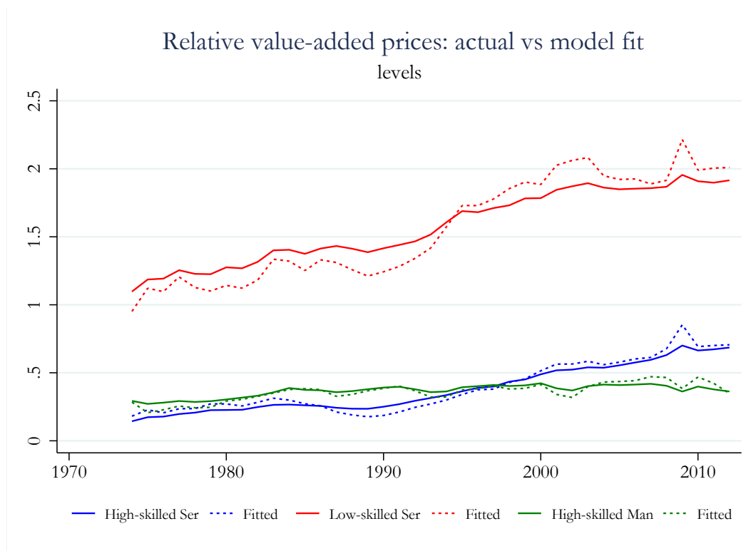
Figure 11: Relative prices
