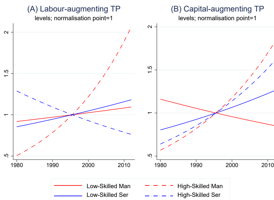
Figure 9: Technical progress
