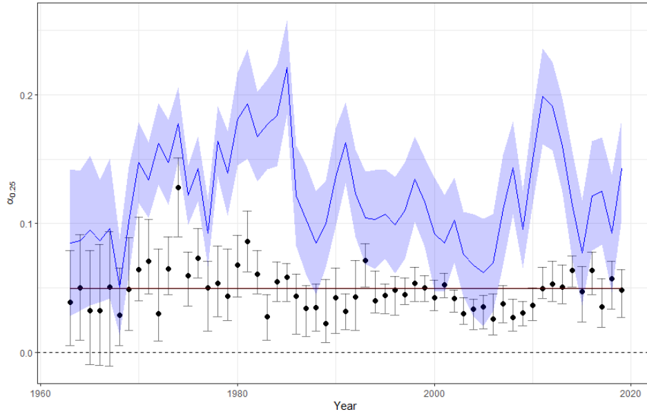
Figure 12: Point estimates time evaluation, blue lines represent cross sectional OLS estimates, black dots represent cross sectional quantile regression estimates and straight line represent pooled quantile regression estimate, \tau = \{0.25\}
