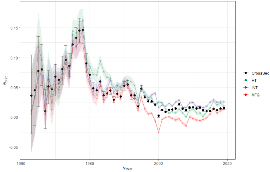
Figure 22: Point estimates time evaluation, sectoral fixed effects, intangible intensive fixed effects, manufacturing fixed effects and high-tech fixed effects presented, \tau = \{0.25\}
