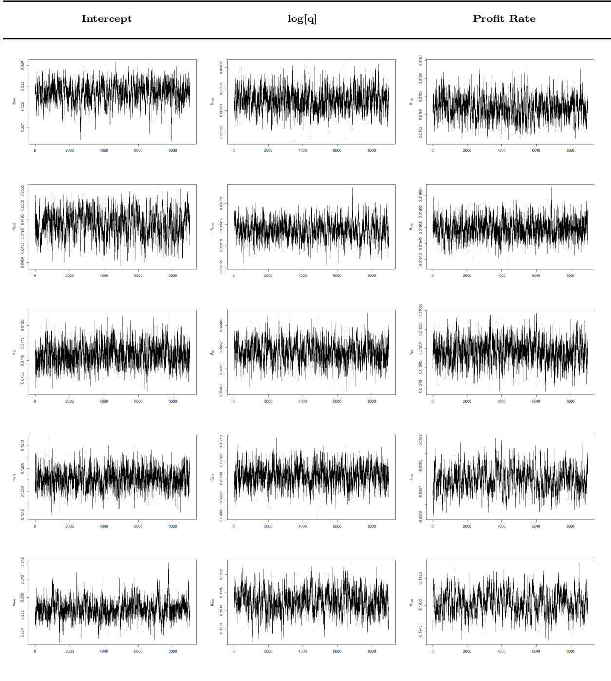
Figure 8: Traceplots of posterior samples from pooled quantile regression model, \tau = \{0.05, 0.25, 0.50, 0.75, 0.95\}
