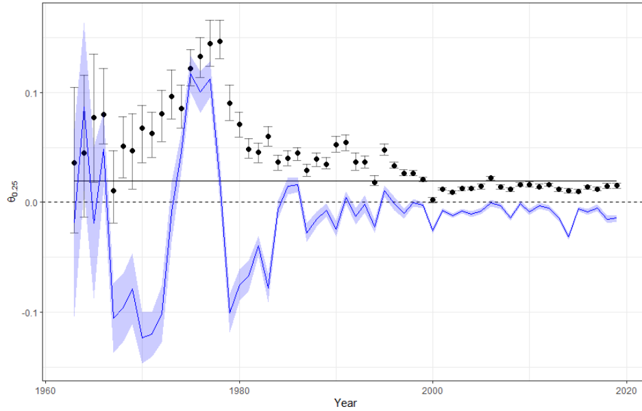
Figure 16: Point estimates time evaluation, blue lines represent cross sectional OLS estimates, black dots represent cross sectional quantile regression estimates and straight line represent pooled quantile regression estimate, \tau = \{0.25\}
