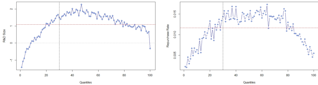
Figure 7: Median Research and Development expenses size and Mean Stock Repurchase Rate of the firms at Investment Rate quantiles
