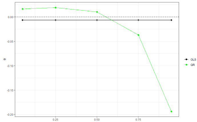
Figure 11: Pooled Quantile Regression estimates of \theta (profit rate) with %90 Credibility Intervals
