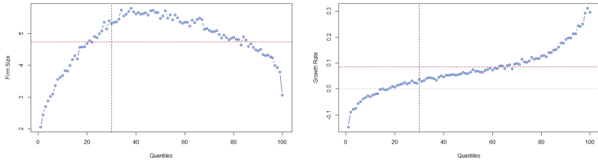
Figure 3: Median Size and Growth rate of the firms at Investment Rate quantiles
