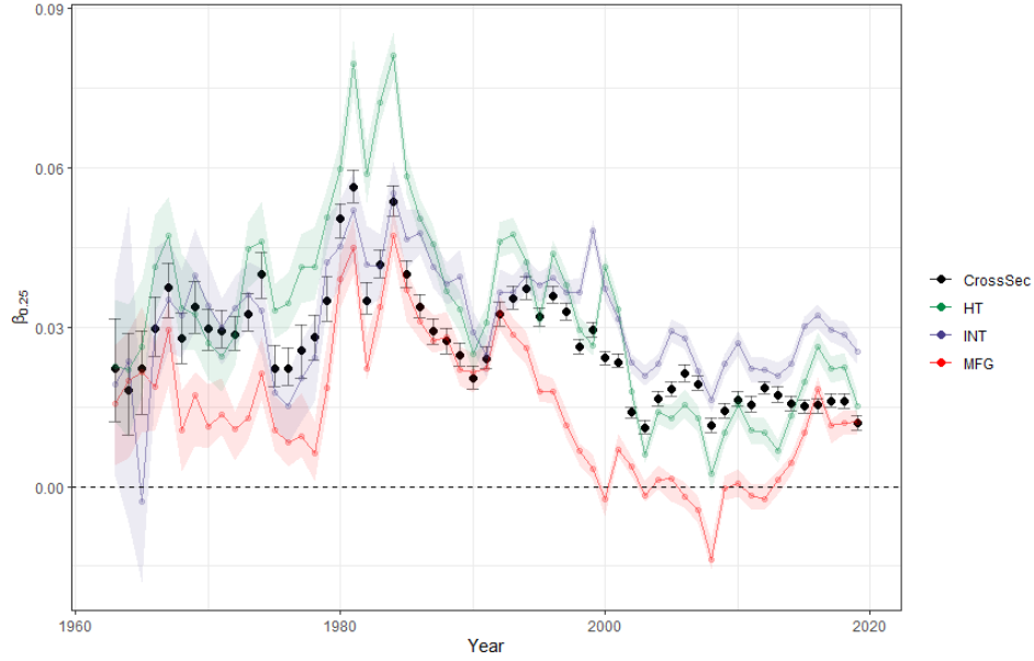
Figure 20: Point estimates time evaluation, sectoral fixed effects, intangible intensive fixed effects, manufacturing fixed effects and high-tech fixed effects presented, \tau = \{0.25\}
