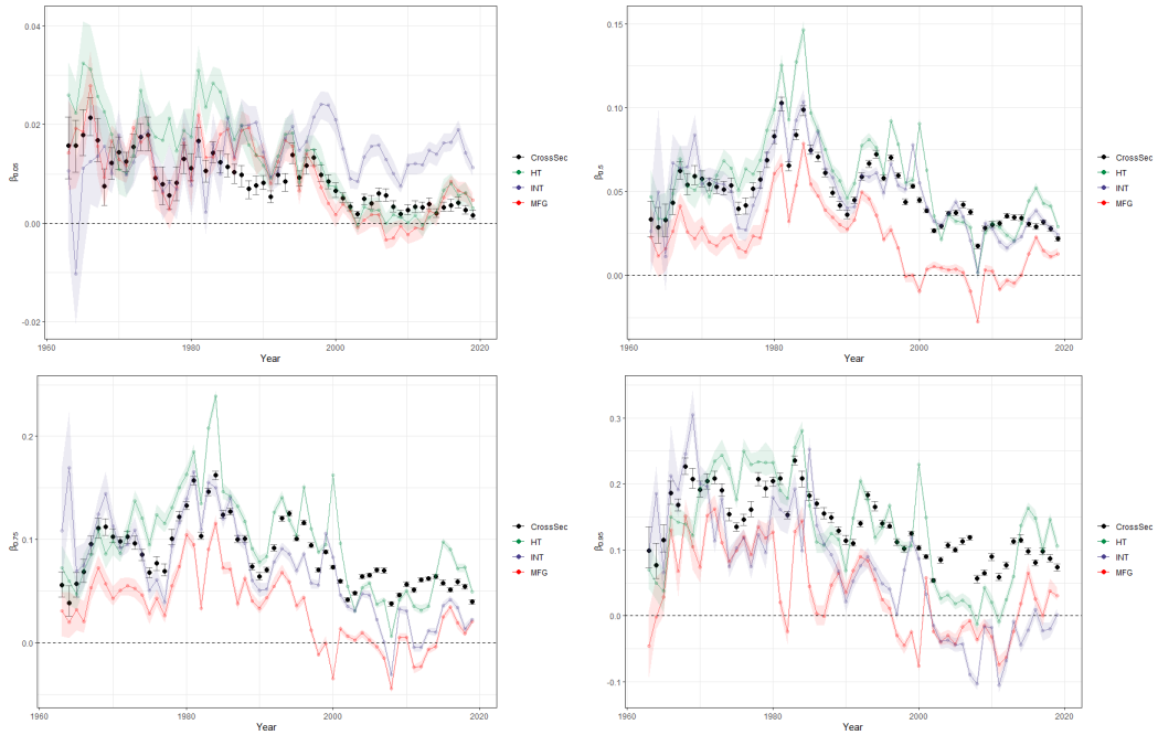
Figure 21: Point estimates time evaluation, sectoral fixed effects, intangible intensive fixed effects, manufacturing fixed effects and high-tech fixed effects presented, \tau = \{0.05, 0.50, 0.75, 0.95\}
