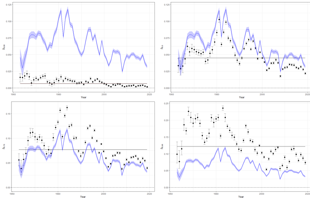
Figure 15: Point estimates time evaluation, blue lines represent cross sectional OLS estimates, black dots represent cross sectional quantile regression estimates and straight line represent pooled quantile regression estimate, \tau = \{0.05, 0.50, 0.75, 0.95\}
