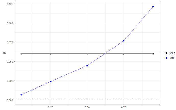
Figure 10: Pooled Quantile Regression estimates of \beta ( \log[q] ) with %90 Credibility Intervals
