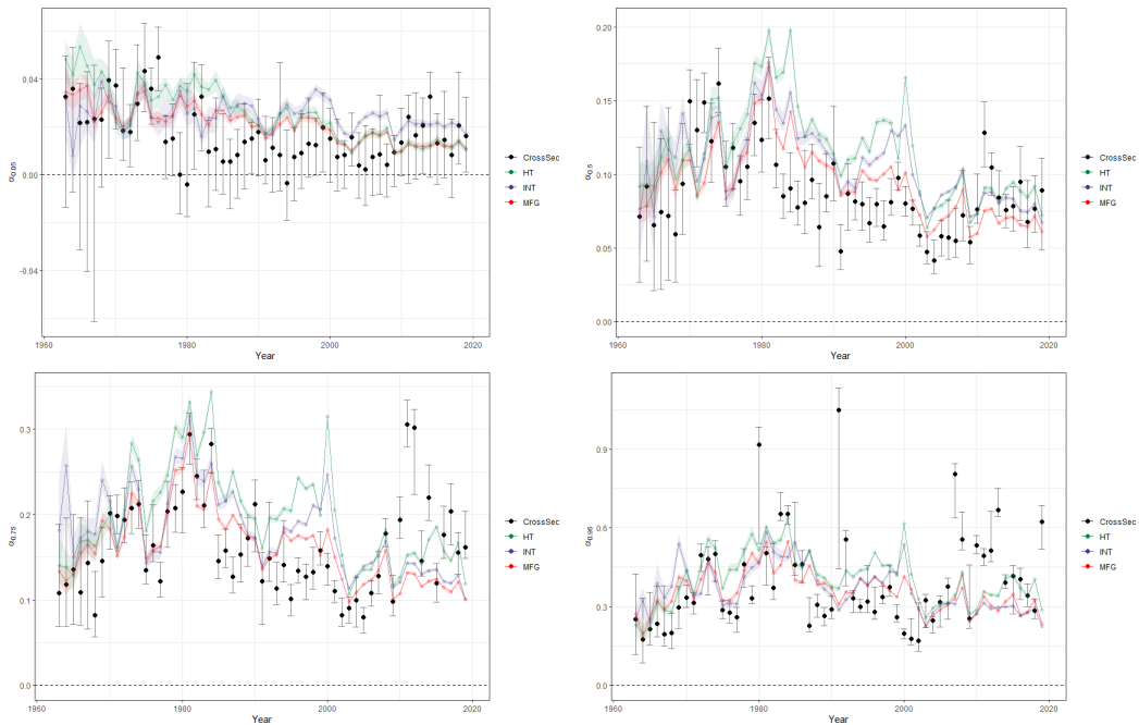
Figure 19: Point estimates time evaluation, sectoral fixed effects, intangible intensive fixed effects, manufacturing fixed effects and high-tech fixed effects presented, \tau = \{0.05, 0.50, 0.75, 0.95\}
