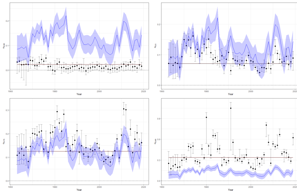
Figure 13: Point estimates time evaluation, blue lines represent cross sectional OLS estimates, black dots represent cross sectional quantile regression estimates and straight line represent pooled quantile regression estimate, \tau = \{0.05, 0.50, 0.75, 0.95\}
