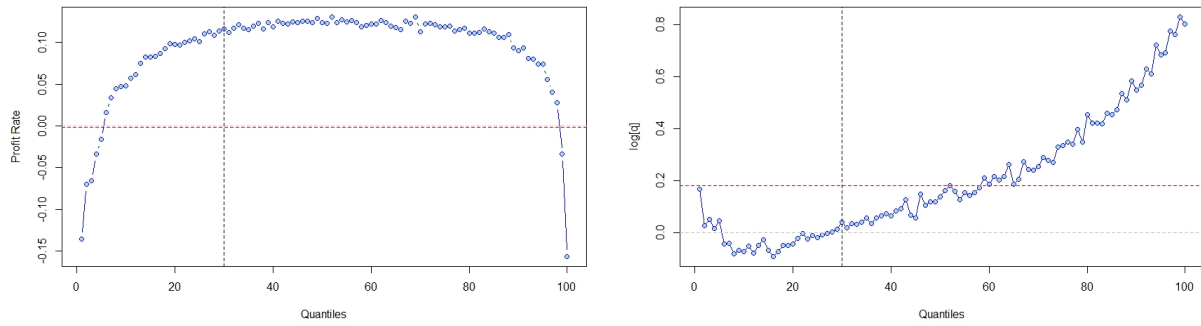
Figure 4: Median Profit Rate and \log[q] of the firms at Investment Rate quantiles
