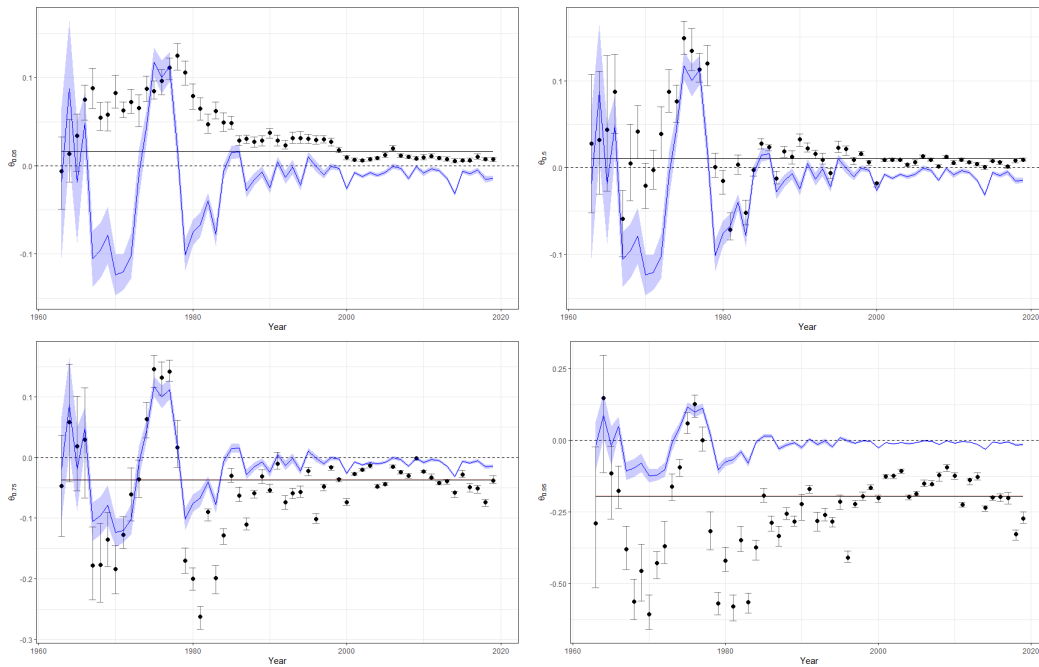
Figure 17: Point estimates time evaluation, blue lines represent cross sectional OLS estimates, black dots represent cross sectional quantile regression estimates and straight line represent pooled quantile regression estimate, \tau = \{0.05, 0.50, 0.75, 0.95\}
