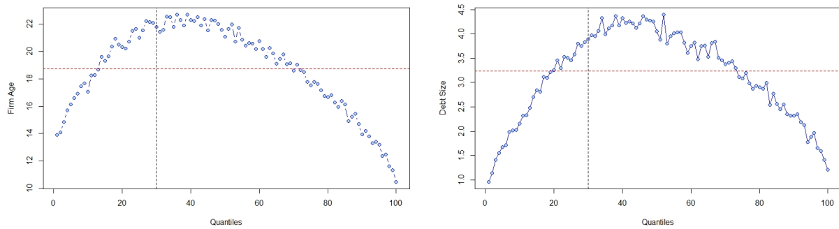
Figure 5: Mean Age and Median Debt Size of the firms at Investment Rate quantiles
