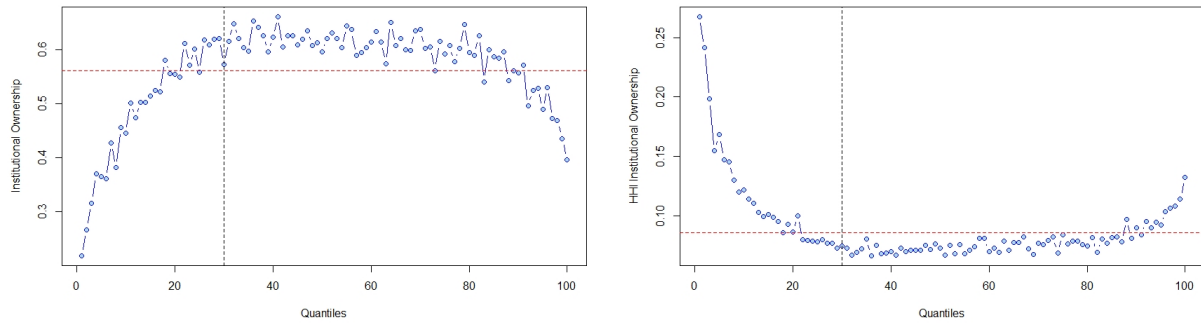
Figure 6: Median Institutional Ownership (%) and HHI of the Institutional Ownership of the firms at Investment Rate quantiles
