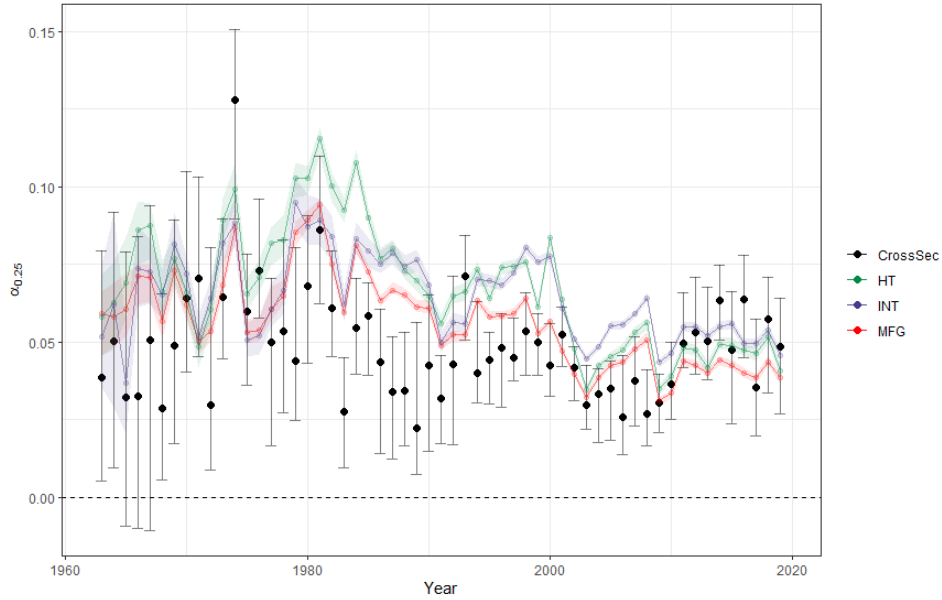
Figure 18: Point estimates time evaluation, sectoral fixed effects, intangible intensive fixed effects, manufacturing fixed effects and high-tech fixed effects presented, \tau = \{0.25\}
