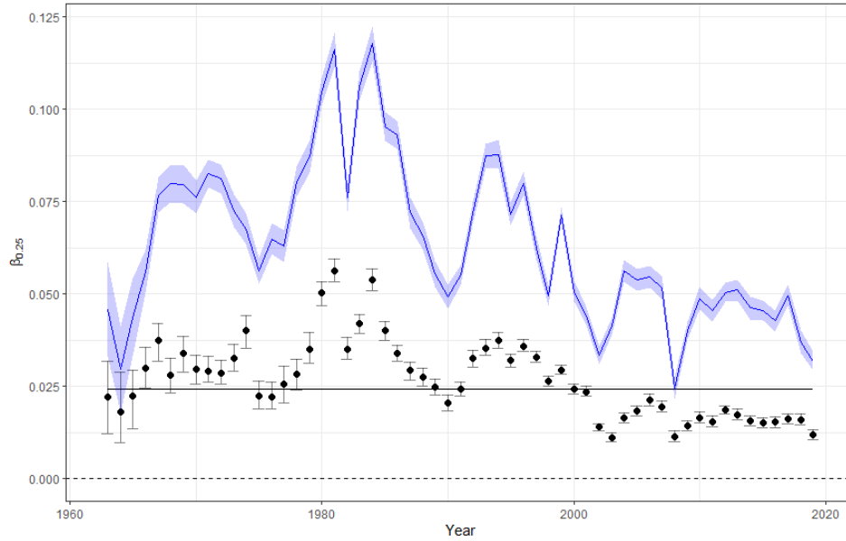
Figure 14: Point estimates time evaluation, blue lines represent cross sectional OLS estimates, black dots represent cross sectional quantile regression estimates and straight line represent pooled quantile regression estimate, \tau = \{0.25\}
