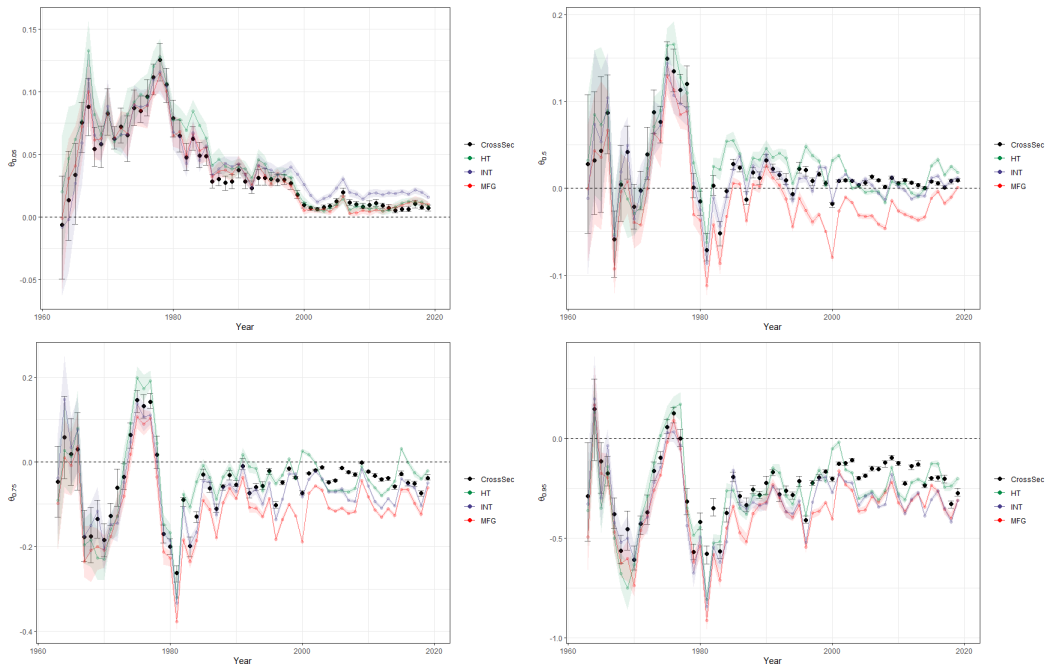
Figure 23: Point estimates time evaluation, sectoral fixed effects, intangible intensive fixed effects, manufacturing fixed effects and high-tech fixed effects presented, \tau = \{0.05, 0.50, 0.75, 0.95\}
