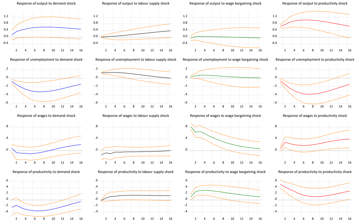
Figure 6: Impulse-responses derived from the SVAR model for the period 1985Q1–2018Q3 (considering all variables in levels). These figures show the impulse-responses obtained from the identification strategy based on model (6). The dynamic responses of the variables to a 1% aggregate demand shock, 1 percentage point labour supply shock, 1% wage bargaining shock and 1% productivity shock are shown in blue, black, green and red, respectively. Orange dotted lines correspond to the respective 95% asymptotic confidence intervals. The horizontal axis shows quarters ahead in all figures.
