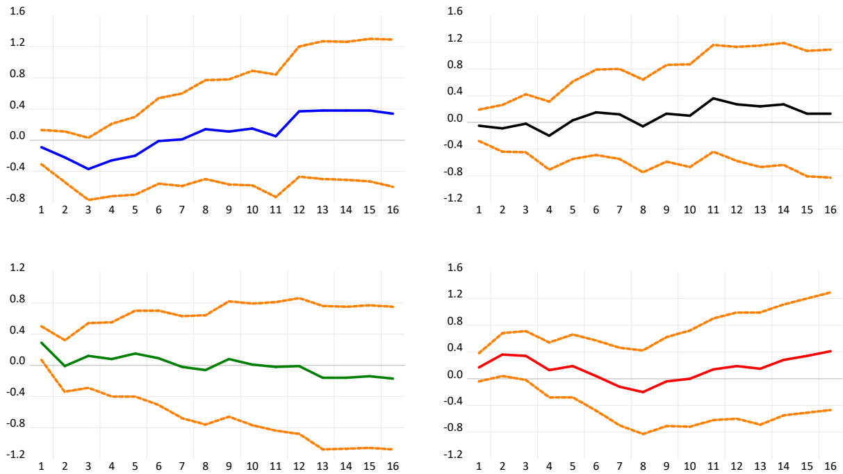
Figure 8: Differences in the responses of the labour share to structural shocks between the subperiods 1948Q1–1984Q4 and 1985Q1–2018Q3. These figures correspond to the responses of the labour share ( \psi_t ) to the structural shocks for the subperiod 1985Q1–2018Q3 minus the ones for the subperiod 1948Q1–1984Q4 (both shown in Figure 7). The differences in the responses of \psi_t to a 1% aggregate demand shock, 1 percentage point labour supply shock, 1% wage bargaining shocks and 1% productivity shocks between both subperiods are shown in blue, black, green and red, respectively. Orange dotted lines correspond to the respective bootstrapped 95% confidence intervals. The horizontal axis shows quarters ahead in all figures.
