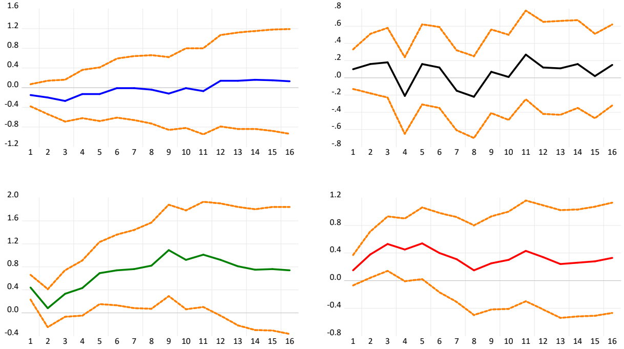
Figure 4: Differences in the accumulated responses of the labour share to structural shocks between the periods 1948Q1–1984Q4 and 1985Q1–2018Q3. These figures correspond to the cumulative responses of the first-differences of the labour share ( \Delta\psi_t ) to the structural shocks for the period 1985Q1–2018Q3 minus the ones for the period 1948Q1–1984Q4 (both shown in Figure 3). The differences in the cumulative responses of \Delta\psi_t to a 1% aggregate demand shock, 1 percentage point labour supply shock, 1% wage bargaining shock and 1% productivity shocks between both subperiods are shown in blue, black, green and red, respectively. Orange dotted lines correspond to the respective bootstrapped 95% confidence intervals (5,000 replications in all cases). The horizontal axis shows quarters ahead in all figures.
