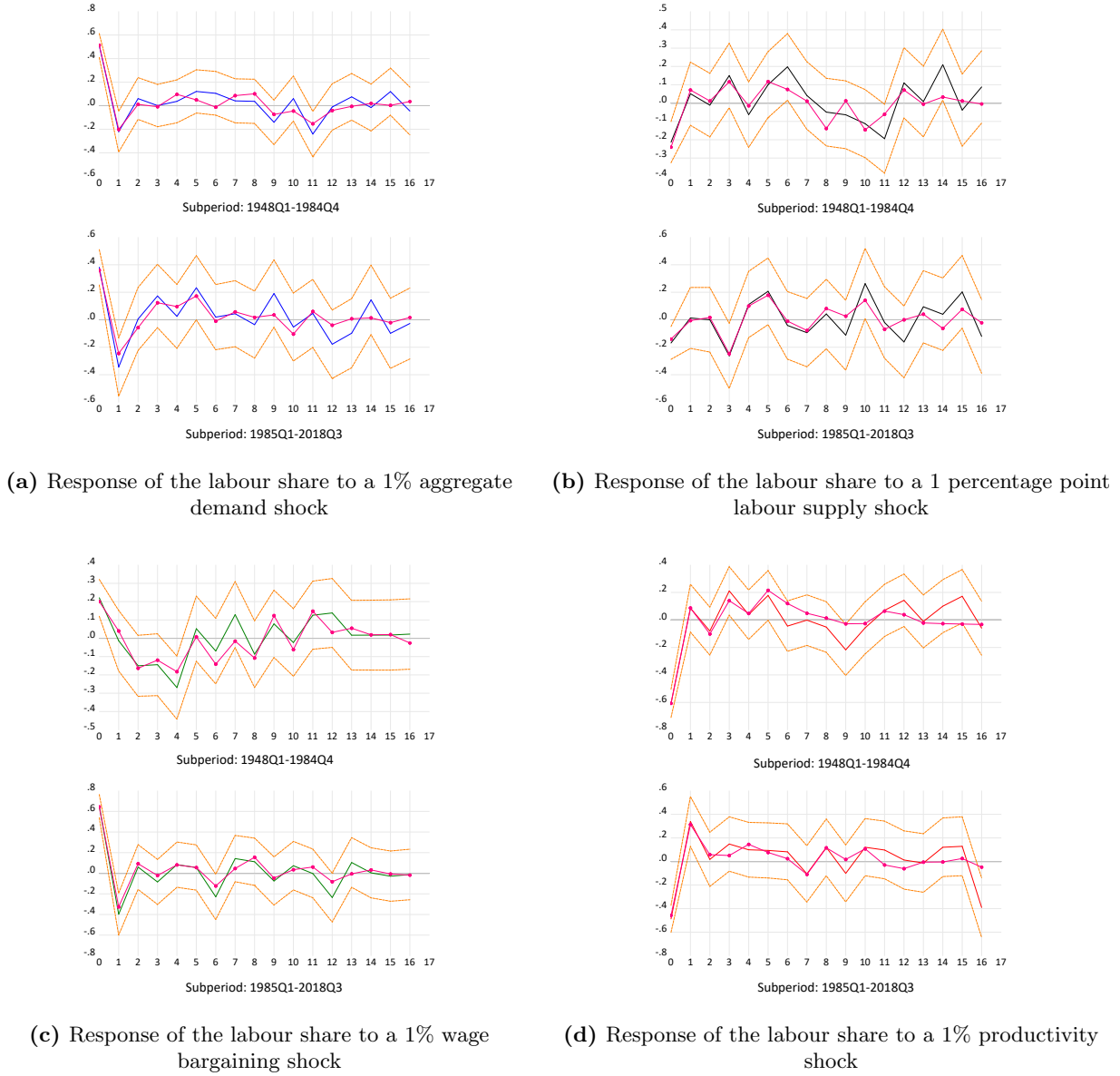
Figure B.1: Comparison of the impulse-responses of the first-differences of the labour share ( \Delta\psi_t ) to structural shocks for the subperiods 1948Q1–1984Q4 and 1985Q1–2018Q3 obtained via local projections and Vector Autoregressions. These figures correspond to the Impulse-Response Functions (IRFs) of \Delta\psi_t with respect to the different structural innovations obtained via local projections and Vector Autoregressions. Orange dotted lines correspond to the respective marginal 95% confidence intervals around the local projections estimates. Pink straight lines with circles correspond to the VAR IRFs used to construct the Cumulative IRFs shown in Figure 3. The horizontal axis shows quarters ahead in all figures.
