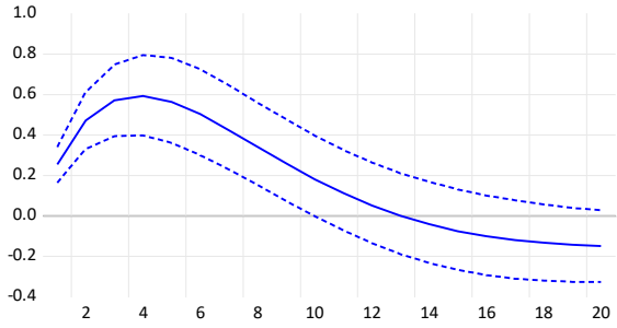
(c) Response of v_t to an i_t shock, 2004Q4
