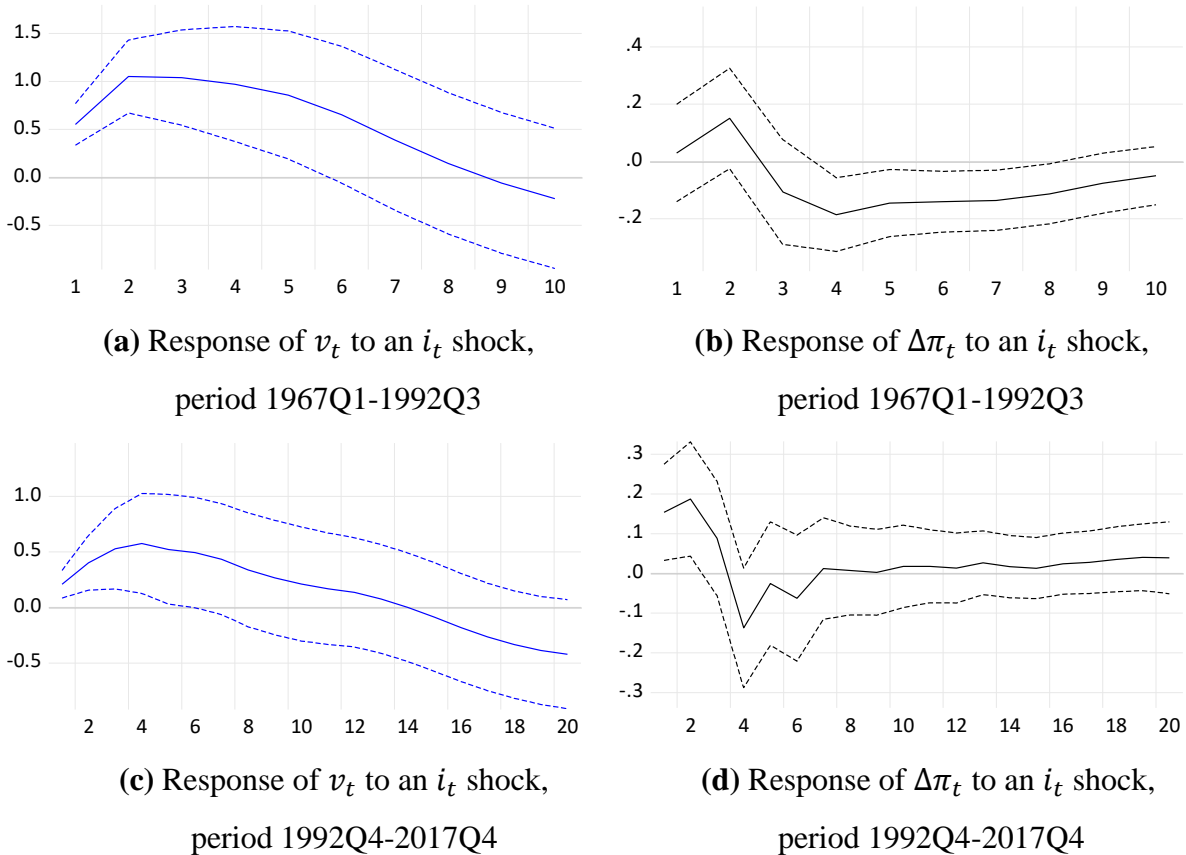
Figure 4. Impulse-response functions obtained from the SVAR models that represent the craft production system’s short-run output adjustment. The VARs for the periods 1967Q1-1992Q3 and 1992Q4-2017Q4 included 3 and 6 lags, respectively. These VAR models did not present problems of serial correlation at the 5% level. The estimated VAR for the period 1992Q4-2017Q4 included an exogenous trend since it was found to be jointly significant according to a Wald coefficient test. Notation: v_t = capacity utilization rate; i_t = investment rate; and \Delta\pi_t = first differences of the natural log of productivity. Dotted lines are the 95% confidence intervals generated via 2,000 Monte Carlo simulations
