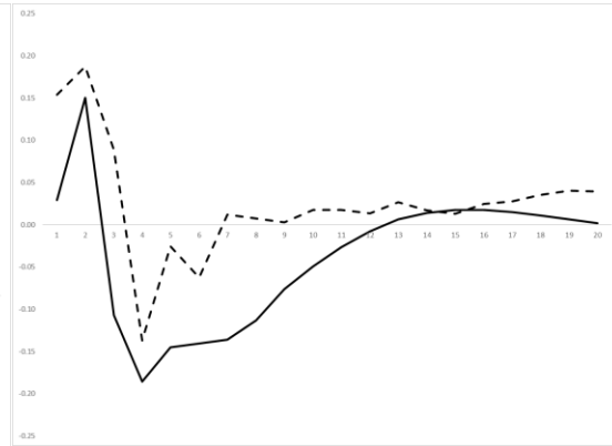
(d) Responses of \Delta\pi_t to an i_t shock, craft production system (Figure 4)
