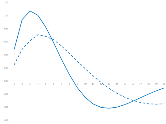
(a) Responses of v_t to an i_t shock, mass production system (Figure 3)
