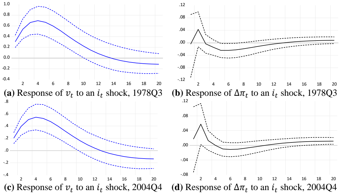
Figure B.4. Impulse-response functions obtained from the TVP-SVAR model that represents the craft production system's short-run output adjustment. Notation: v_t = capacity utilization rate; i_t = investment rate; and \Delta\pi_t = first differences of the natural log of productivity. Dotted lines are the 68% confidence intervals
