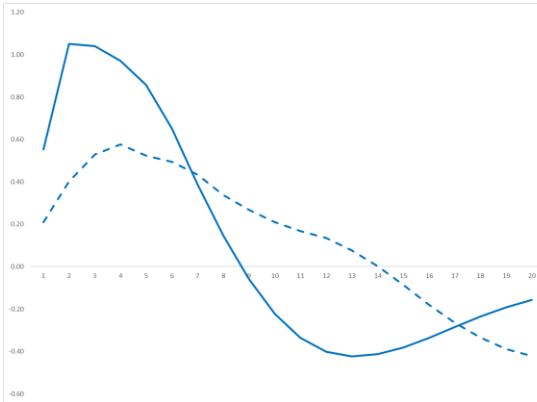
(c) Responses of v_t to an i_t shock, craft production system (Figure 4)
