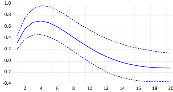
(a) Response of v_t to an i_t shock, 1977Q3
