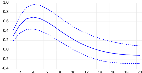
(a) Response of v_t to an i_t shock, 1978Q3
