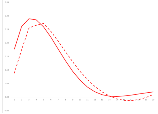
(b) Responses of n_t to a v_t shock, mass production system (Figure 3)
