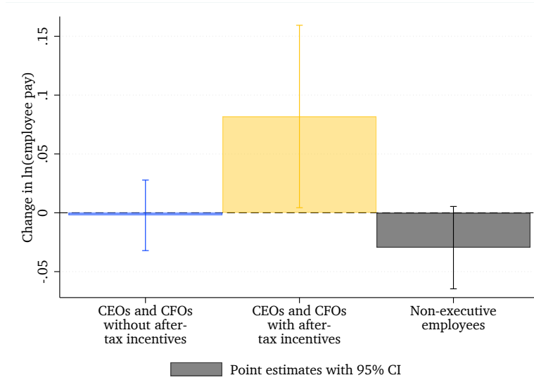
FIGURE 6 – Benchmark results
