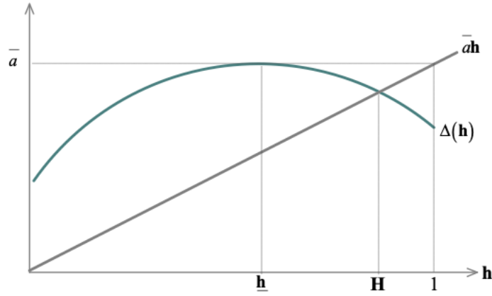
Figure 10: \underline{\mathbf{h}} < \mathbf{H} < 1
