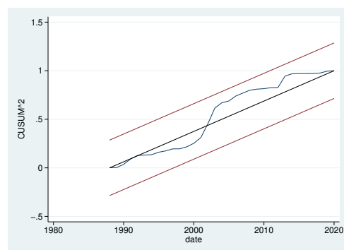
(b) Gold CUSUM squared test
