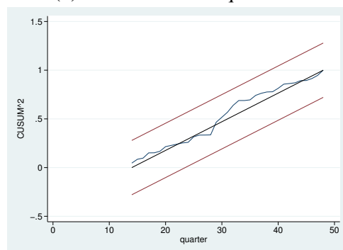
(f) Bitcoin CUSUM squared test
