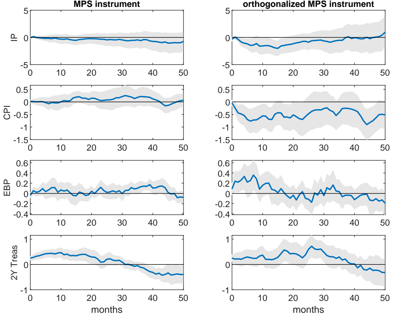
Figure 5: Local Projections
