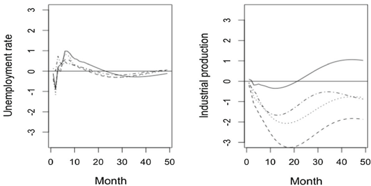
Fig. 26 The impulse response functions of unemployment rate and industrial production estimated using different time windows. The dot-dashed lines represent impulse response functions estimated using the data from January 2008 to July 2017, dashed lines from January 2009 to July 2017, dotted lines from February 2009 to July 2017 and solid lines from May 2009 to July 2017
