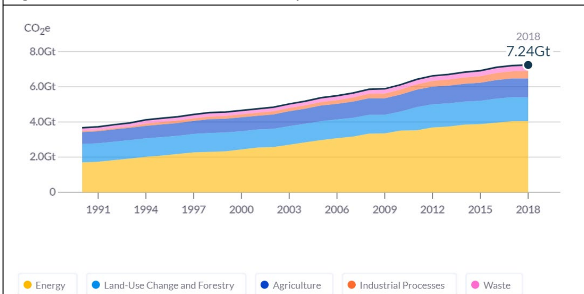
Figure 2: Evolution of Africa's GHG emissions by sector, 1990-2018
