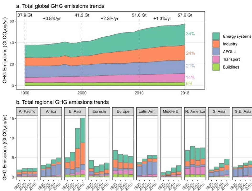
Figure 1: Global and regional GHG emissions by sector, 1990-2018
