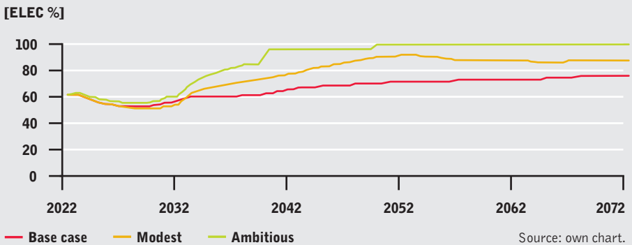
Fig. 2f: Summary of the simulation results Electricity from renewable %
