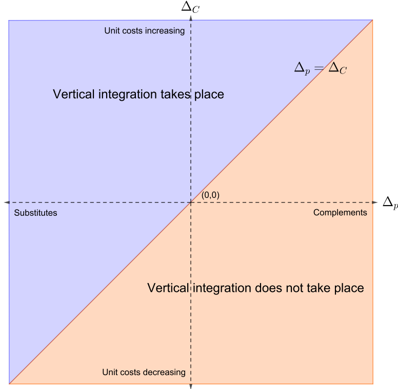
Figure 1: Vertical integration incentives
