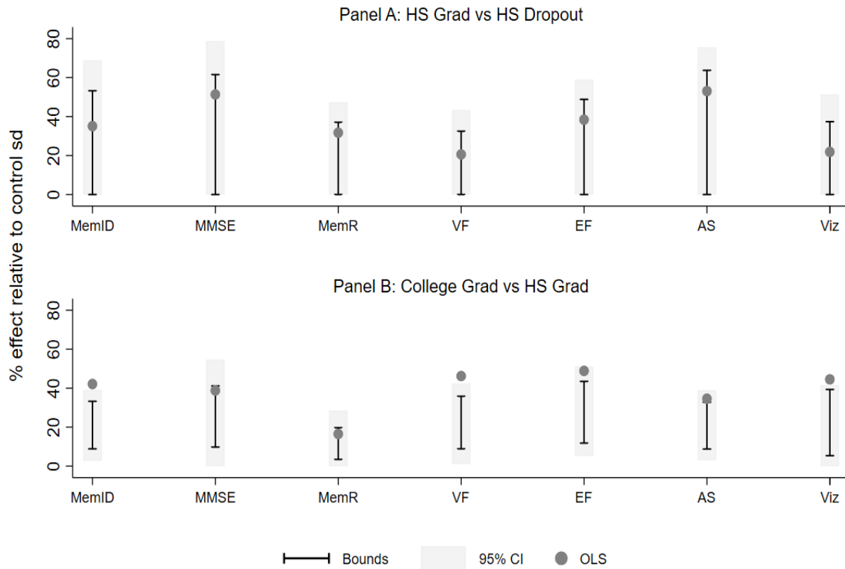
Figure 4: Inverse Probability Weightaged MTS+MTR+MIV Bounds and OLS Estimates
