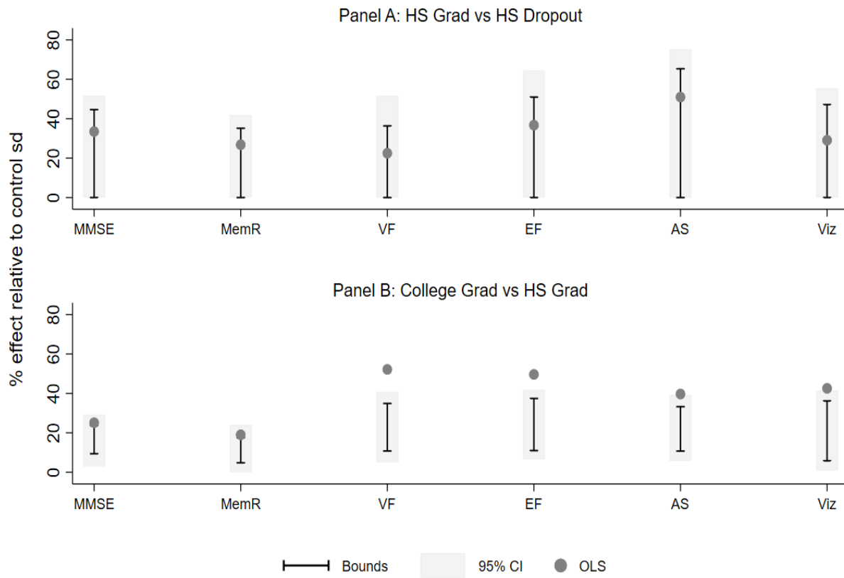
Figure 2: MTS+MTR+MIV Bounds for Other Cognition Domains
